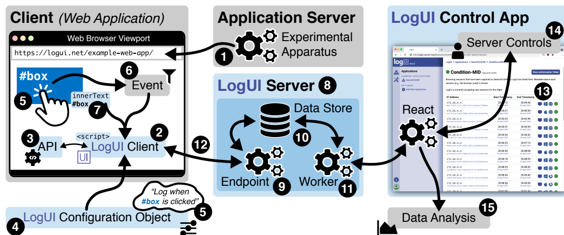
Figure 3: Architectural diagram of LogUI. Blue boxes denote components specific to LogUI; refer to §3.2 for more information. Circled numbers are used throughout §3 to highlight certain concepts; these pertain to the numbers in the illustration above.
