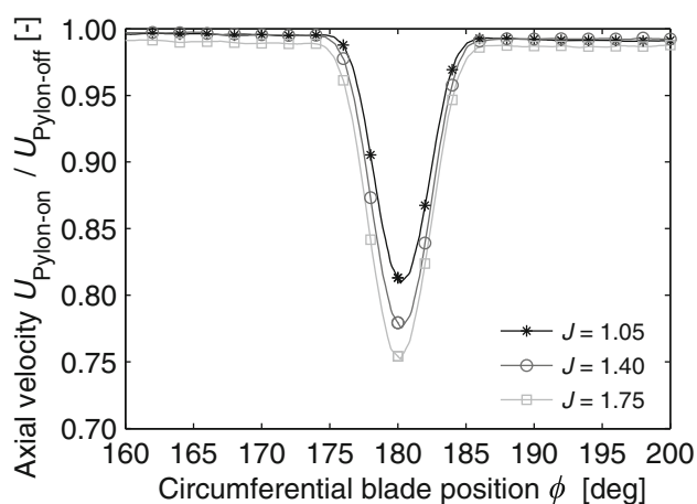
Fig. 5 Effect of propeller thrust setting on the wake velocity deficit experienced by a blade section at r/R = 0.65 , 0.078D upstream of the propeller, \beta = 0^\circ
