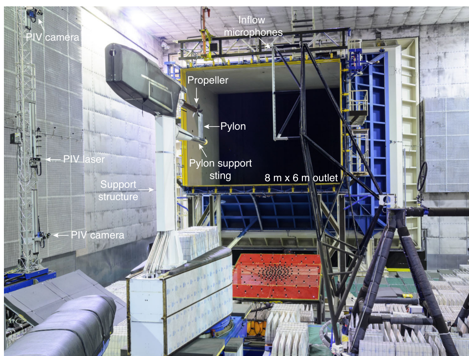
Fig. 1 Photograph of the experimental setup, showing the propeller and pylon models, acoustic instrumentation, and PIV system
