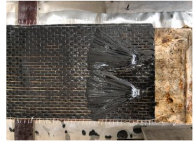
(c) Bonding of the CFRP sheet and anchors with epoxy resin
