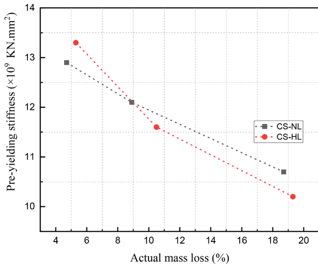
Fig. 12. Pre-yielding stiffness curves.
