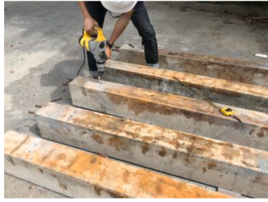
(a) Concrete drilling
