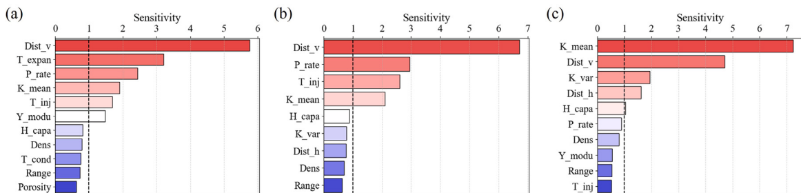
Fig. 9. Sensitivity analysis results of responses, with parameters having a sensitivity value over 1 classified as sensitive (including all sensitive parameters and the top 5 insensitive parameters): (a) stability of the drift, (b) temperature at the drift, (c) temperature at the production well.
