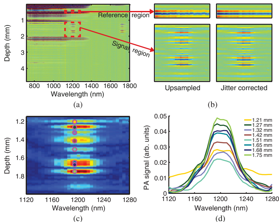
Fig. 3 Spectroscopic intravascular photoacoustics (sIVPA) data processing to obtain depth-resolved IVPA spectra. (a) Band pass filtered PA traces at different wavelengths. Regions containing the tissue (bottom rectangle) and reference (top rectangle) signals are indicated. (b) Upsampling and jitter correction. (c) Light intensity-corrected data in the tissue signal region with colored circles marking peaks above a certain threshold in the signal envelope of the PA trace at 1195 nm. (d) Resulting spectra at those sites after noise filtering.
