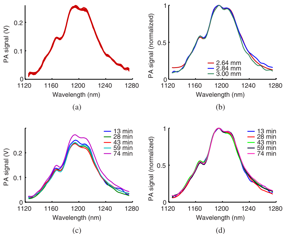
Fig. 5 Robustness of lipid PA spectroscopy showing data from cholesterol linoleate as an example. (a) Comparison of "single-shot" spectra. (b) Spectra obtained at different depths. (c) Evolution of the spectral amplitude over time. (d) Data from panel (c) after normalization.
