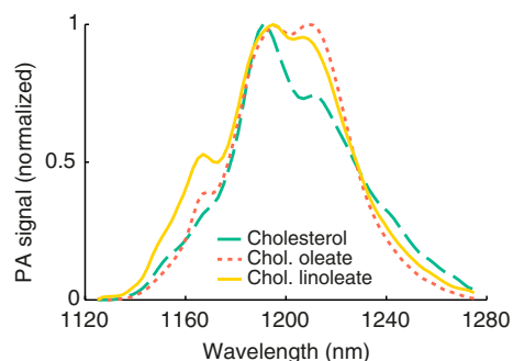
Fig. 4 Absorption spectra of cholesterol, cholesterol oleate, and cholesterol linoleate in the 1200-nm wavelength region as recorded by PA spectroscopy exhibit clear differences.
