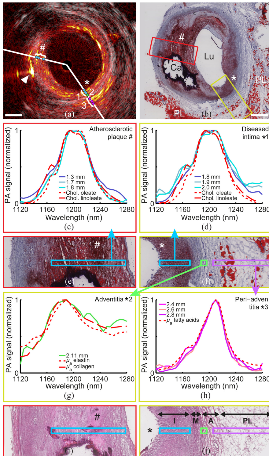
Fig. 6 IVPA spectra of a human atherosclerotic coronary artery, ex vivo . (a) Dual-modality IVPA/IVUS image, arrowhead indicates suture needle. Along the white lines (# and *), spectral IVPA data were obtained. Normalized IVPA spectra at the locations of the dots are shown in (c) (#, blue dots), (d) (*, blue dots), (g) (*, green dot), and (h) (*, purple dots), compared to absorption spectra obtained in Fig. 4 and reference spectra for collagen, elastin, and fatty acids from literature. 29 (b) Histology section of the site imaged in (a), showing near circumferential intimal lipid accumulation (red) and presence of a calcification (Ca). The lipid rich core (#) and pathological intimal thickening (PIT; *) are magnified (3×) in (e) and (f), respectively, showing the locations where the IVPA spectral data are recorded. (i) Hematoxylin–Eosin (H&E) histologic stain of the area #, showing reduced cellularity in the plaque. (j) H&E stain of the area *, showing PIT and an intact media. Spectra locations in (c), (d), (g), and (h) are stated in millimeter from the catheter tip. Oil Red O stain, Lu = lumen, PL = peri-adventitial lipid. Scale bars indicate 1 mm. Dynamic range of IVPA and IVUS image is 40 dB; color scales as in Fig. 2.
