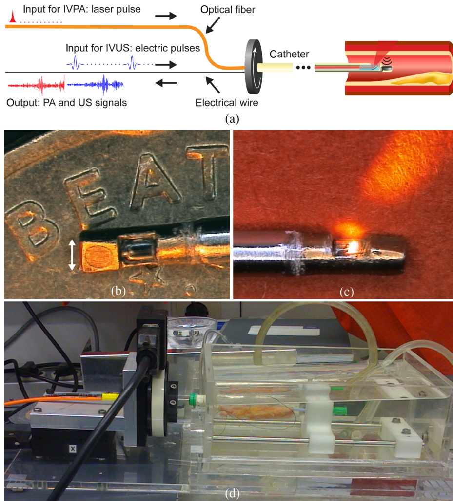
Fig. 1 Combined intravascular photoacoustics (IVPA) and intravascular ultrasound (IVUS) imaging. (a) The intravascular IVPA/IVUS catheter is inserted in an ex vivo human coronary artery and rotated in 1 deg steps. Laser pulses for IVPA imaging and electric pulses for pulse echo (IVUS) imaging are delivered to the vessel wall interleaved at every angular position. (b) Photograph of the catheter tip on the edge of a 10 eurocent coin. White arrow indicates 1 mm. (c) Photograph of the catheter tip, showing the light beam exiting the catheter. (d) Photograph of artery in setup, side view. On the left, the translation ( x ) and rotary stage are visible.
