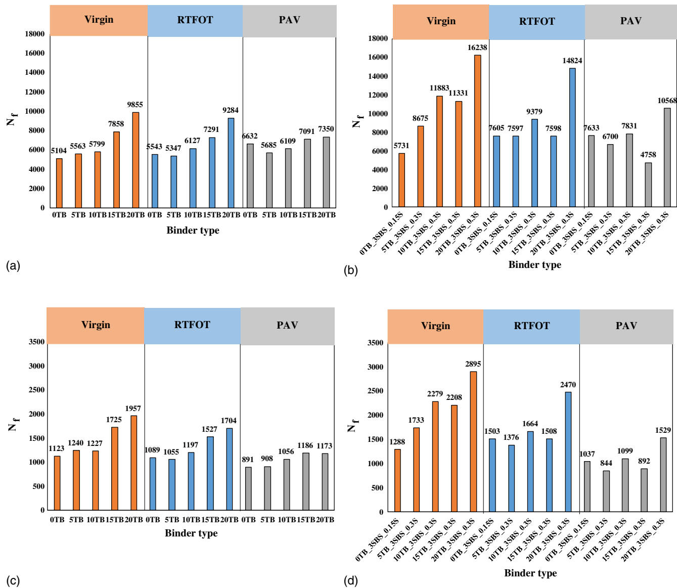
Fig. 11. Fatigue life before and after aging at different strain levels: (a) TBRA at 2.5% strain; (b) TBHA at 2.5% strain; (c) TBRA at 5% strain; and (d) TBHA at 5% strain.
