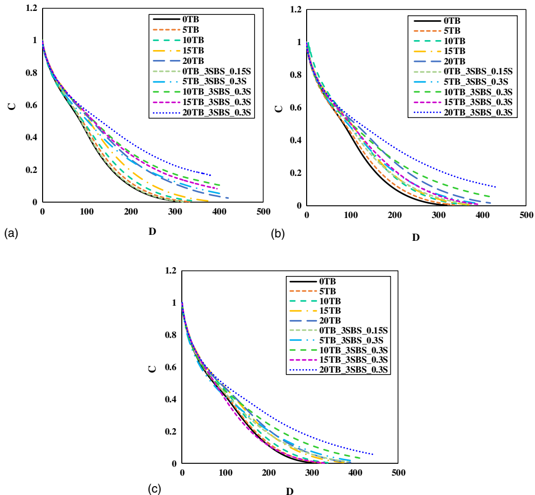
Fig. 9. Damage characteristic curves under different aging conditions (a) virgin; (b) RTFOT; and (c) PAV.
