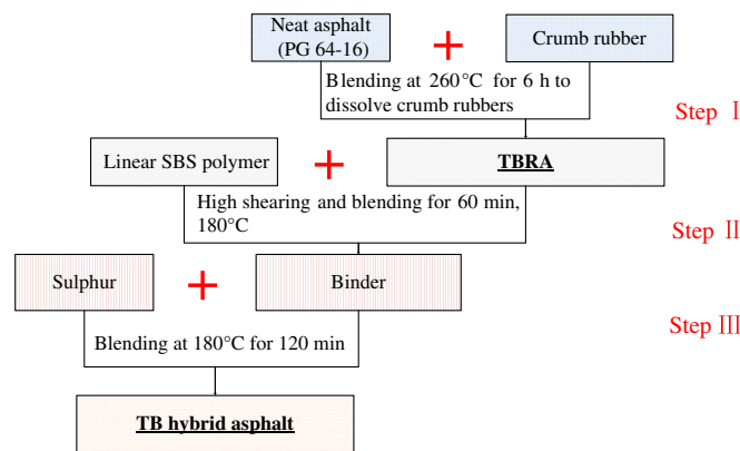
Fig. 1. Schematic of binder preparation.
