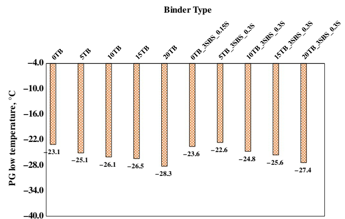
Fig. 7. Binder PG low-temperature grades.
