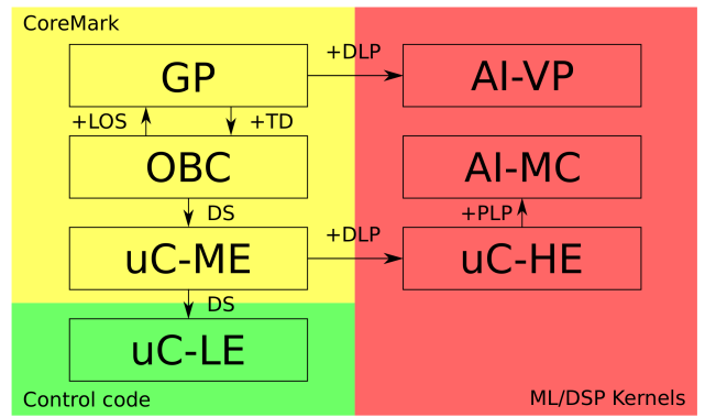
Figure 1. Identified profiles of processors for space applications, main differences among them and defining benchmarks. LOS stands for "Support for Linux-like OSs", DS stands for "Downsized", TD for "Time Determinism".
