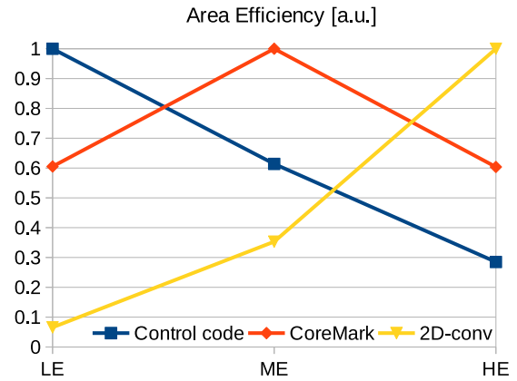
Figure 3. Comparison of the three profiles of microcontrollers targeting different applications (data is from [11], where LE is Zero-risic, ME is Micro-risic and HE is RI5CY). For each benchmark, data is normalized to the achieved peak. 2D-conv stands for “2D-convolution kernel”.
