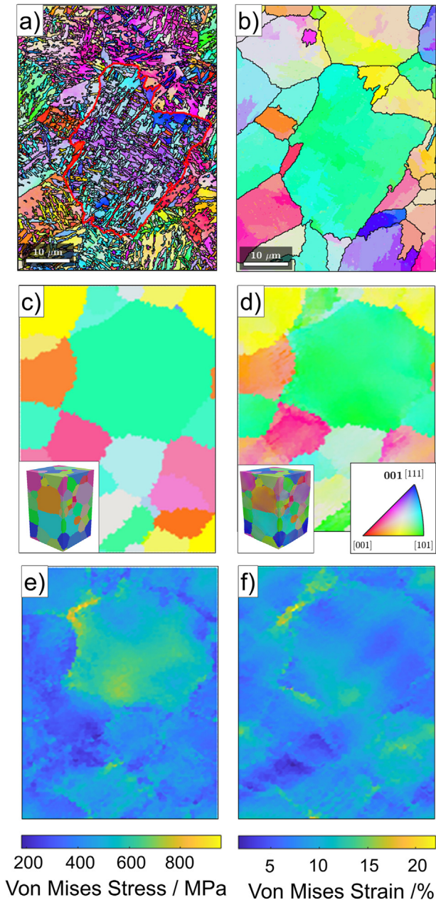
Fig. 10 – (a) Cropped bainitic ferrite Inverse Pole Figure (IPF) EBSD map corresponding to Region 2, T_{def} = 400 °C; (b) Cropped reconstructed austenite Inverse Pole Figure (IPF) EBSD map corresponding to Region 2, T_{def} = 400 °C which was mimicked to be simulated by Damask; (c) middle YZ section of the initial (pre-deformation) RVE, to be compared with subfigure (b) and (on the left bottom) whole initial (pre-deformation) RVE, with IPF coloring; (d) middle YZ section of the final (post-deformation) RVE and (on the left bottom) whole final (post-deformation) RVE, with IPF coloring, where the legend is on the right bottom; (e) Von Mises Stress distribution in the middle YZ section of the RVE; (f) Von Mises Strain distribution in the middle YZ section of the RVE. The compression direction is always vertical.
