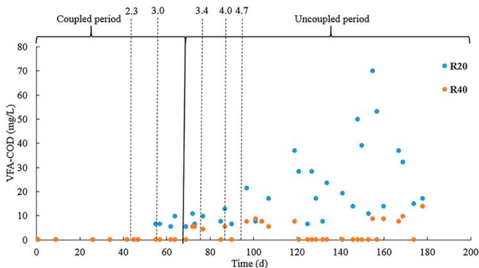
Figure 3. VFA-COD effluent concentration over operational time.
