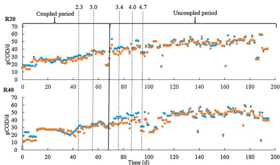
Figure 4. COD mass balance.
