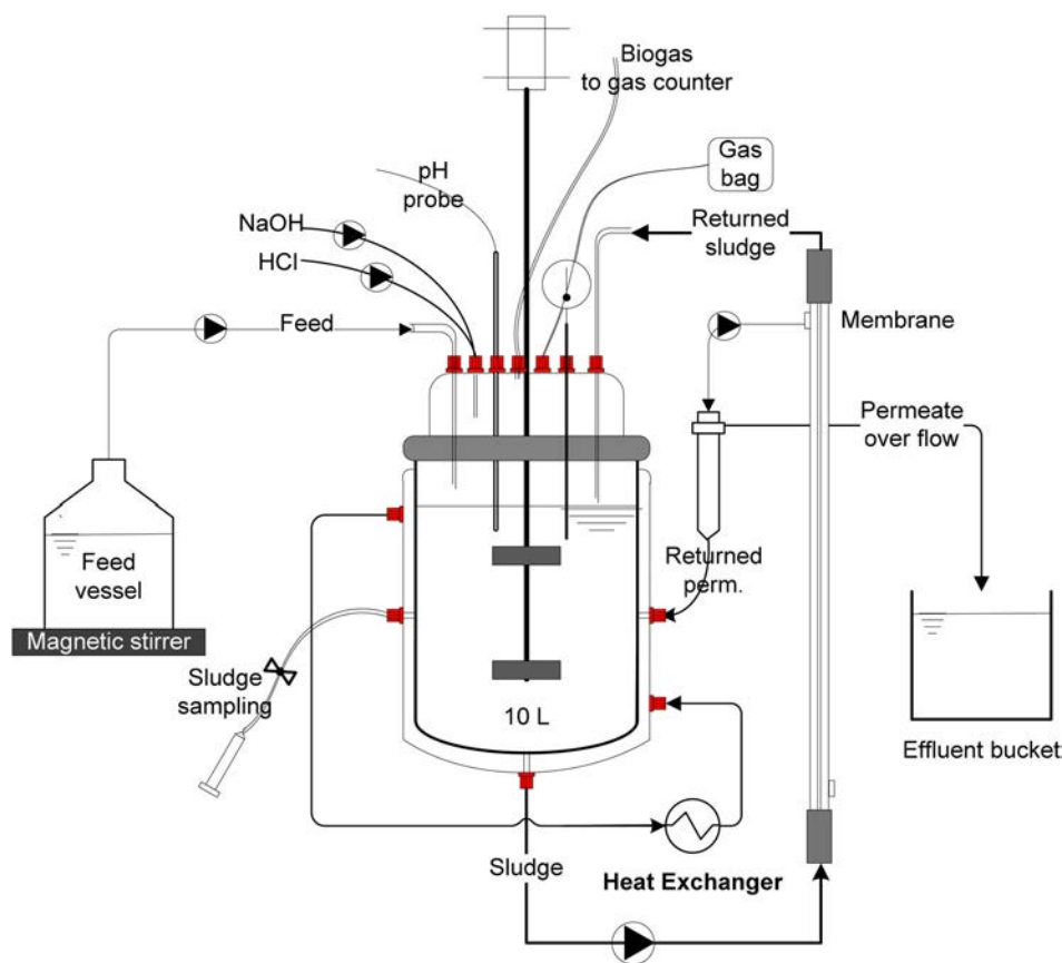
Figure 1. Experimental set-up.
