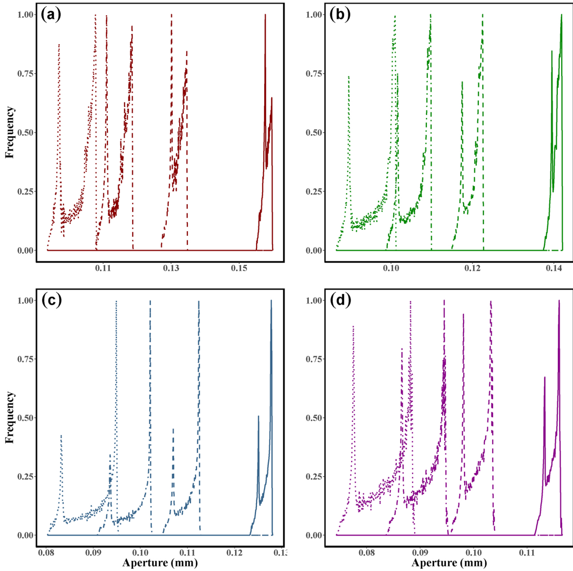
Fig. 5. Fracture aperture distribution for different well pressures – dotted, dotdash, dashed, and solid lines represent p_{wf} = 500, 1000, 1500 , and 2000 psi, respectively: rectangular fracture with (a) 0^\circ , (b) 30^\circ , (c) 45^\circ , and (d) 60^\circ orientation ( \theta ) model. Aperture at initial reservoir pressure for 0^\circ, 30^\circ, 45^\circ , and 60^\circ orientation is 0.233, 0.195, 0.168 and 0.148 mm, respectively, and aperture at well pressure for each well pressure case is located at lower bound of that case.
