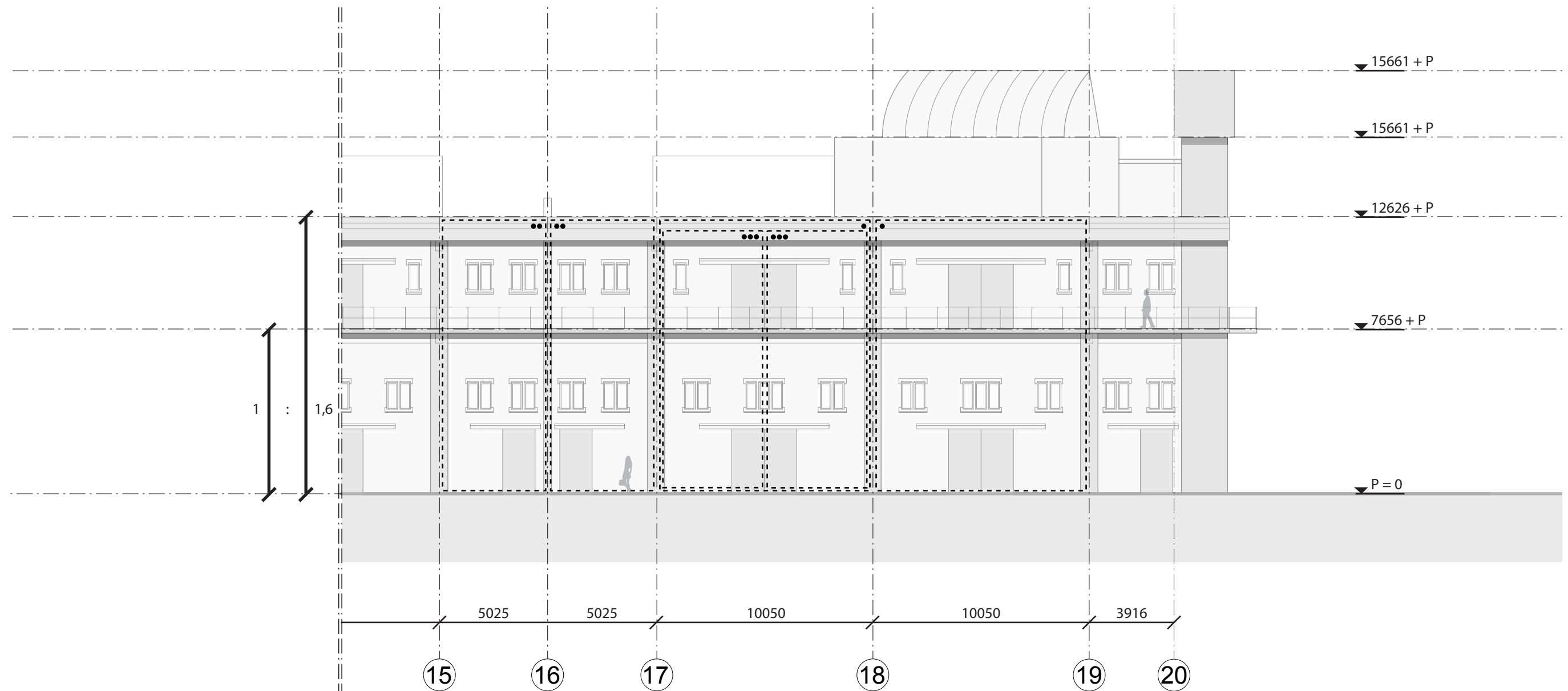
south facade elevation 4 by Jan Huis in 't Veld (own illustration)
