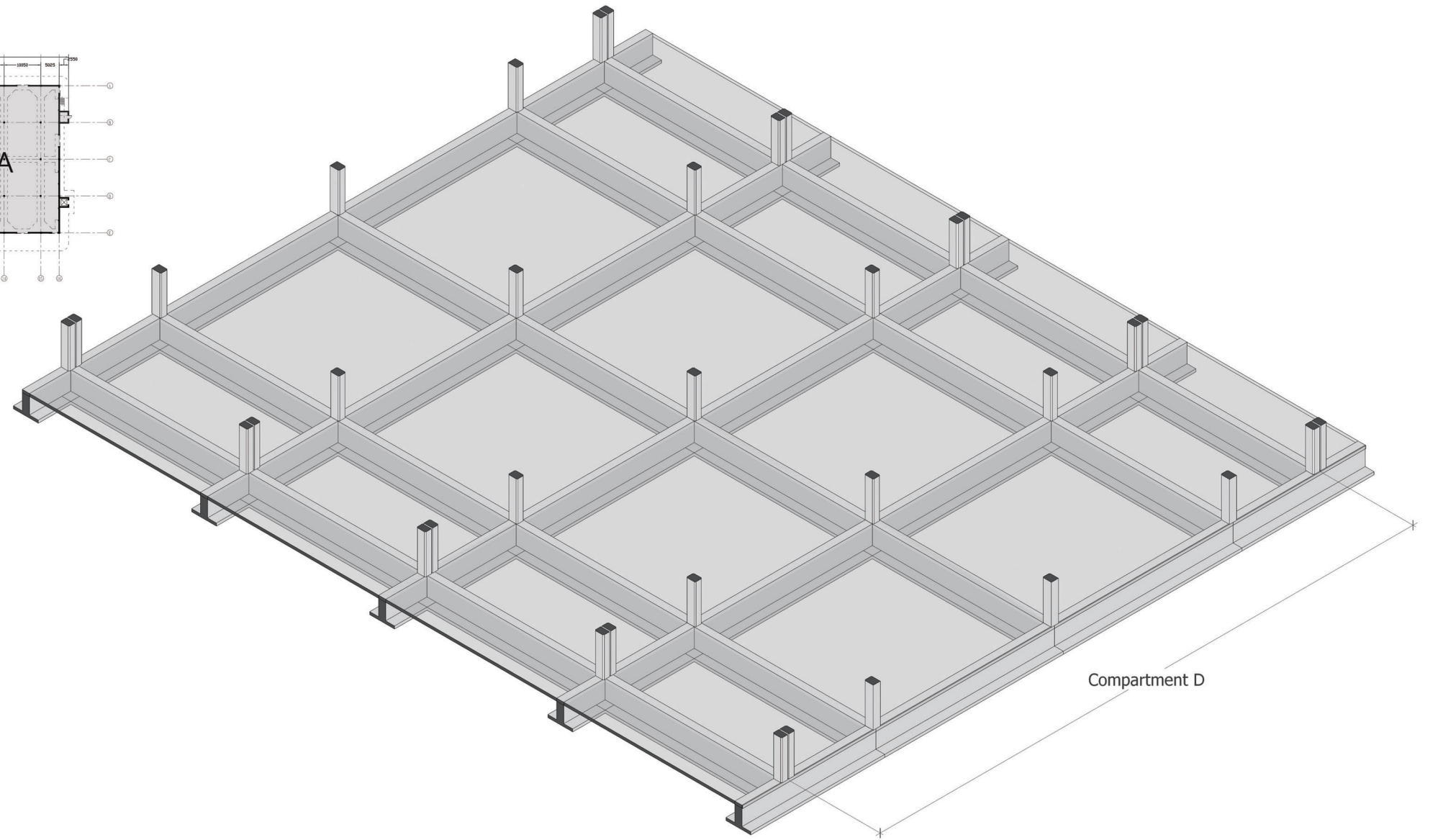
Axonometric view of foundation
