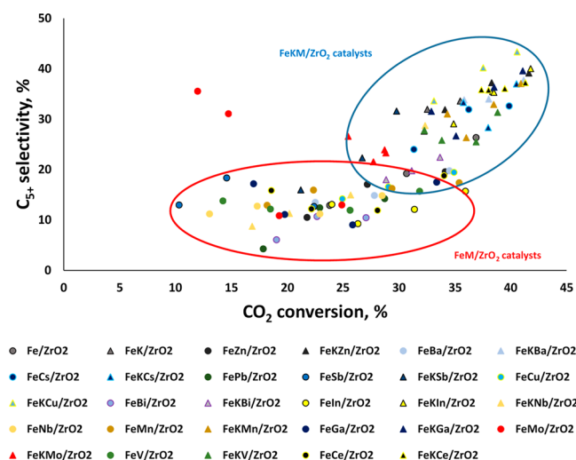
Figure 6. C_{5+} selectivity versus carbon dioxide conversion for Fe/ ZrO_2 promoted catalysts. T = 350\text{ }^{\circ}\text{C} , H_2/CO = 3 , WHSV = 4.67\text{--}18.19\text{ L/g}\cdot\text{h} , P = 10\text{ bar} , TOS = 50\text{ h} .
