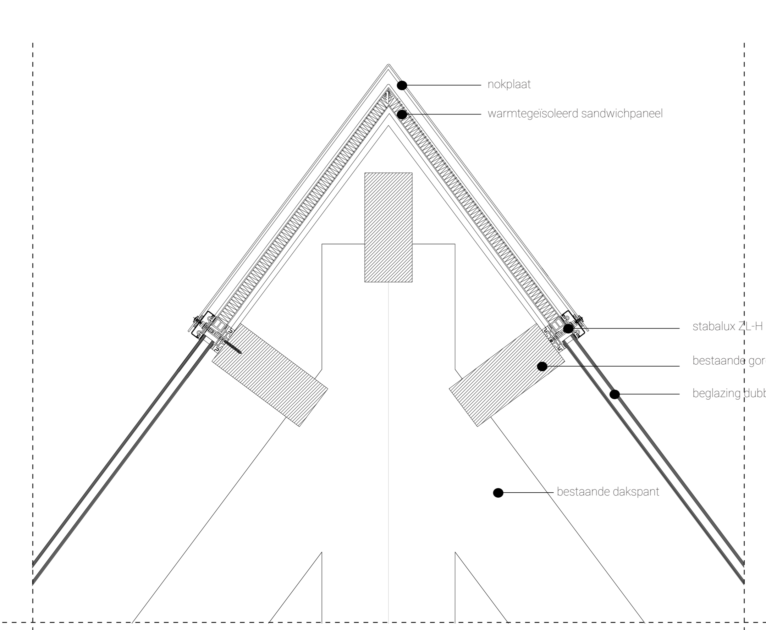
Details dakkas 1:5
