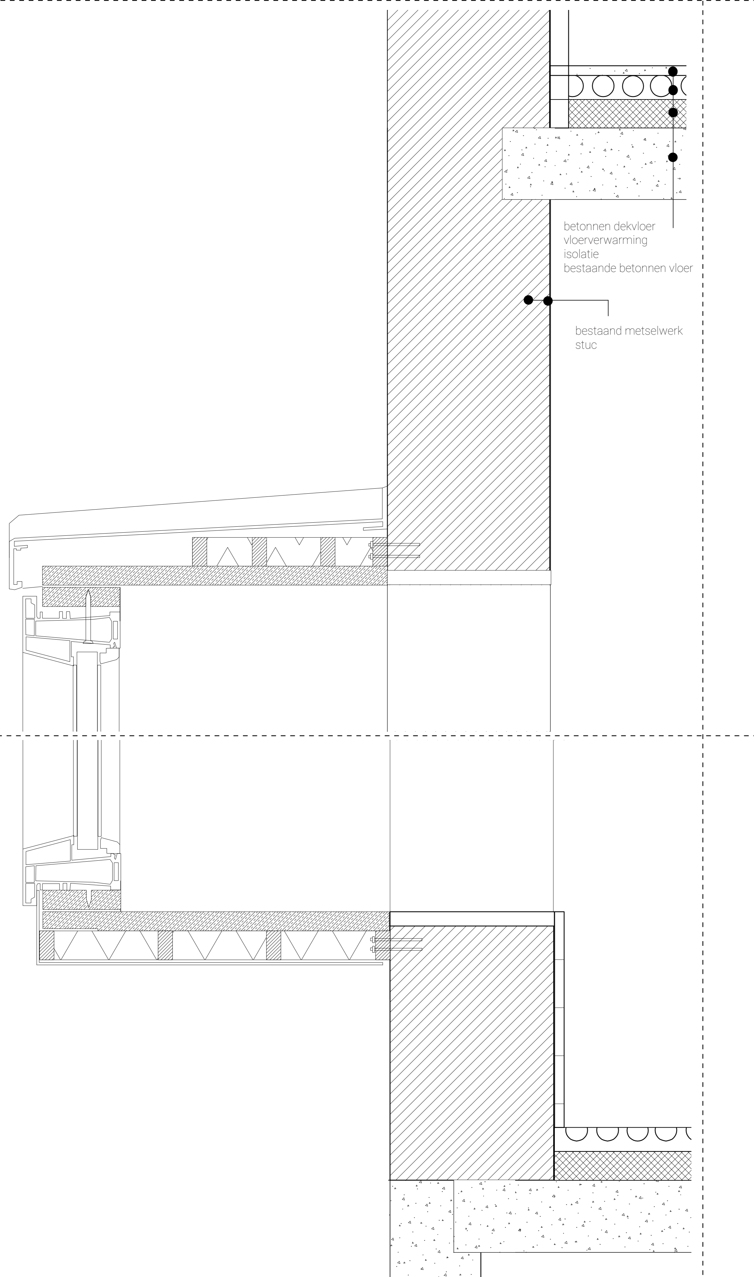
Details baywindow 1:5
