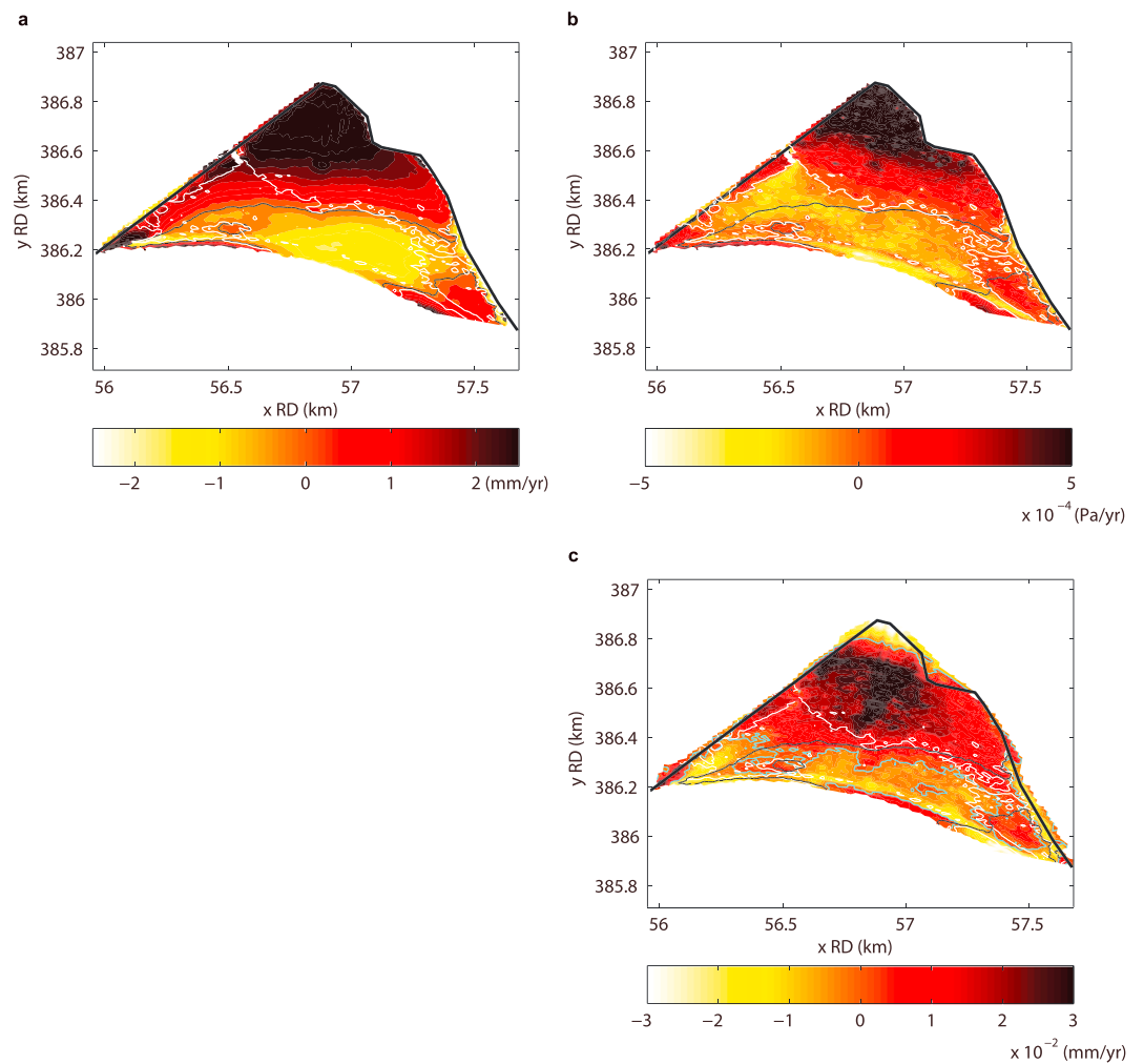
Figure 9. (a) Bed level changes over the first 300 years of the modeled evolution (accretion over time is positive), normalized to millimeters per year. (b) Corresponding changes in the tidally averaged bed shear stress (Pa/year). At most locations, the figure shows a positive correlation between the bed level and the erosion rates, which suggests a negative (stabilizing) internal feedback mechanism. (c) Corresponding changes in averaged wave height in shallow waters (less than 1 m deep), normalized to millimeters per year (with cyan zero-contour lines). (a–c) The thin black and white lines are zero-contour lines of the changes in the bed level and the erosion flux, respectively.
