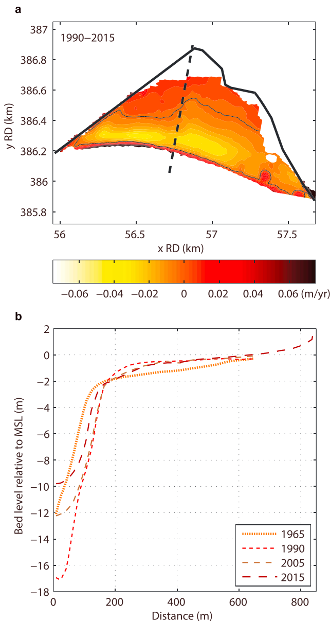
Figure 3. Observed long-term trend on the Kapellebank (based on the Vaklodigen data set; Wiegmann et al., 2005; see also de Vet et al., 2017). (a) Bed level differences, indicated in yearly averages (m) over the period 1990–2015. The black dashed lines indicate the position of the cross-shore transects of panel b. (b) Snapshots of the cross-shore transects in the period 1965–2015. The Kapellebank steepened over the last 25 years. In the last decade, the intertidal bathymetry is relatively stable, despite the large sedimentation rates inside the channel.
