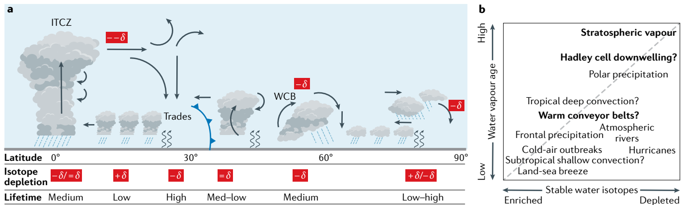
Fig. 4 | The relation between water vapour residence time and stable isotope composition in atmospheric water vapour. a | Schematic depiction of water vapour pathways within global weather systems (including evaporation, transport, mixing and precipitation) and their corresponding approximate lifetime and connection to loss of isotopically heavy vapour during condensation processes. b | Expected correspondence of lifetime to loss of heavy isotopes from weather systems that produce precipitation and residual vapour (bold). Stable water isotopic composition experiences variations during the life cycle of the rain-producing process. While subdaily samples show that synoptic systems can undergo variations across the enriched–depleted spectrum, daily and longer-term samples would provide information on the event peak. ITCZ, Intertropical Convergence Zone; WCB, warm conveyor belt.
