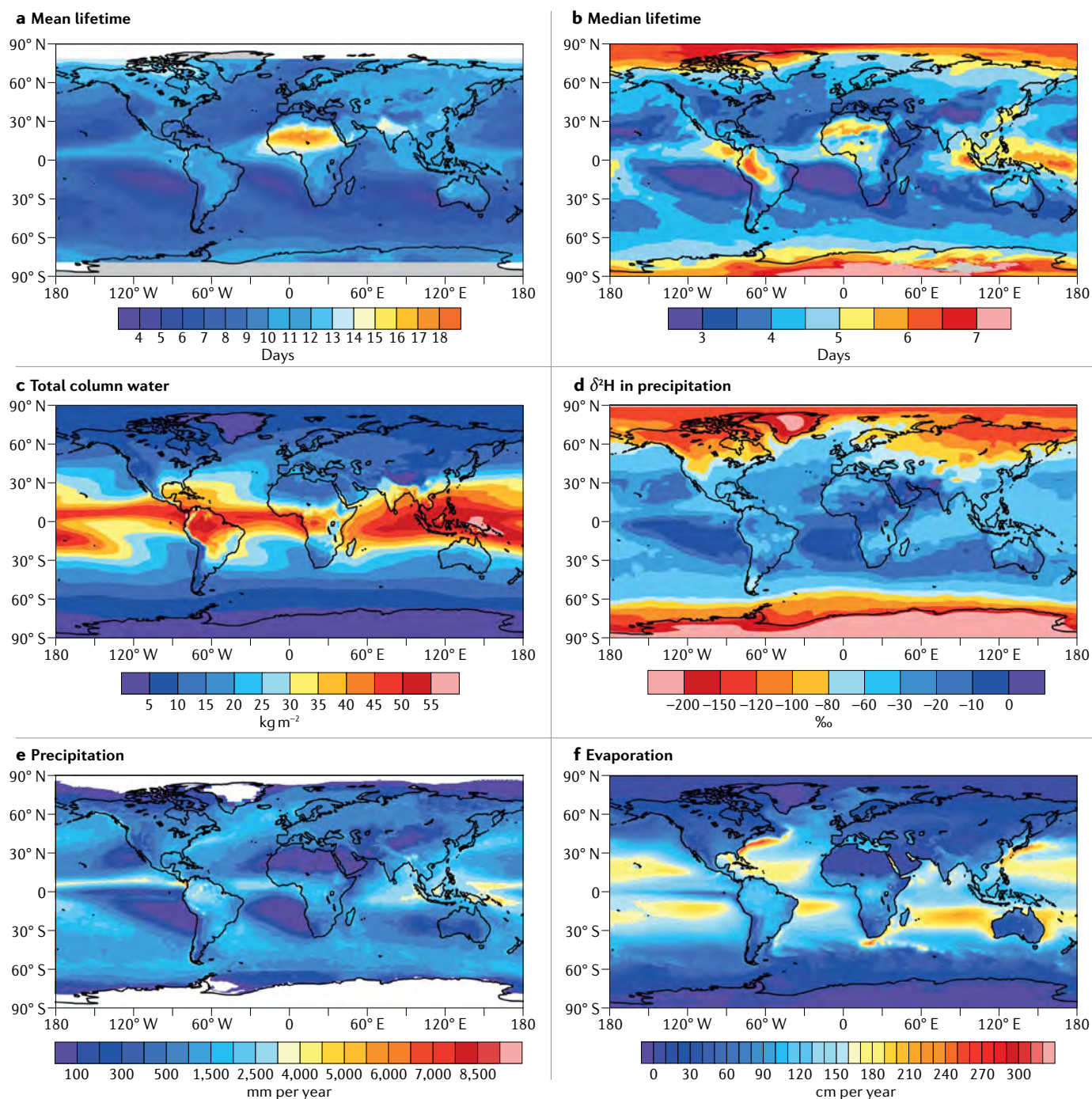
Fig. 3 | Global patterns of water vapour residence time estimates and precipitation characteristics. a | Annual mean lifetime or backward transit time. b | Annual median lifetime or backward transit time. c | Total column water climatology (1980–2019) from ERA5 (REF. 108 ). d | Annual mean \delta^2\text{H} in surface precipitation, as simulated by the isotope-enabled ECHAM5-WISO 109 . e | Annual rainfall total climatology (2001–2019) from 3IMERGM 110 . f | Annual evaporation climatology (1980–2019) from ERA5 (REF. 108 ). The global distribution of mean and median lifetime differs owing to different processes and time scales considered. Panel a adapted from REF. 9 , CC BY 3.0 ( https://creativecommons.org/licenses/by/3.0/ ). Panel b adapted from REF. 7 , CC BY 3.0 ( https://creativecommons.org/licenses/by/3.0/ ).
