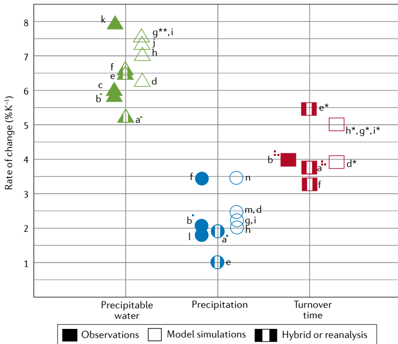
Fig. 5 | Sensitivity of water vapour residence time and its components to global temperature. Rate of change per degree warming for precipitable water (green), precipitation (blue) and turnover time (red). Where needed, turnover time was converted to units % K -1 . *Derived from changes in global precipitable water and precipitation. **Results from AR4 models. ■ Derived from % per decade, with a warming reference of 0.17 K per decade. ■■ Derived from recycling rate. a = REF. 13 ; b = REF. 12 ; c = REF. 83 ; d = REF. 74 ; e = REF. 78 ; f = REF. 75 ; g = REF. 77 ; h = REF. 73 ; i = REF. 72 ; j = REF. 82 ; k = REF. 84 ; l = REF. 107 ; m = REF. 88 ; n = REF. 87 . Note, results from REF. 111 are not included, owing to problems with the underlying precipitation data. Most estimates, whether observational, modelled or hybrid, converge on rates of change close to 7% K -1 for global precipitable water, 2.5% K -1 for global precipitations and about 4.5% K -1 for turnover time.
