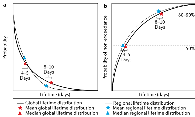
Fig. 1 | Schematic depiction of the global lifetime distribution. a | Probability density functions of lifetime distribution (LTD), or backward transit times depending on terminology, for the globe and a regional example with higher contribution from short-lived vapour. Triangle and star symbols denote the median and mean LTD, respectively, with the latter also representing turnover time. b | As in panel a , but the corresponding cumulative distribution function of the LTD, providing the probability of non-exceedance. While the median LTD is defined as the mid-point of the distribution, the mean LTD is found at variable locations on the upper tail (here, 80–90% of the distribution). LTDs are heavily skewed, vary regionally and can be characterized by their mean or median. Adapted from REF. 7 , CC BY 4.0 ( https://creativecommons.org/licenses/by/4.0/ ).
