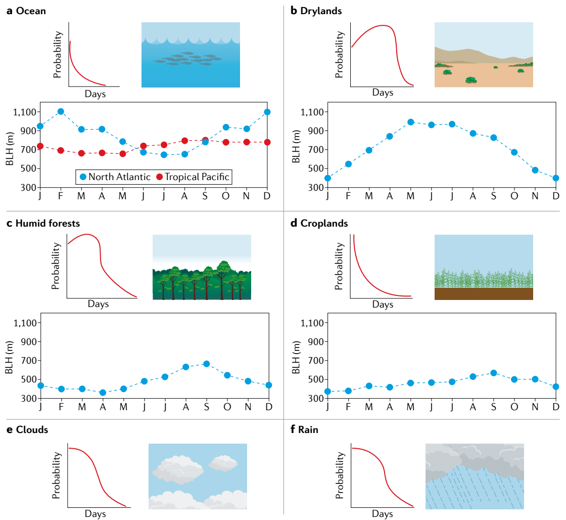
Fig. 2 | Lifetime distribution of different surface conditions and water cycle components. Schematic lifetime distribution (LTD) and boundary layer height (BLH) for ocean (panel a), drylands (panel b), humid forests (panel c), croplands (panel d), clouds (panel e) and rain (panel f). LTDs are roughly based on the findings of REFS 6,37 . BLH values are monthly 2019 averages from ERA5 (REF. 108 ) taken over: 25°–50° N, 15°–60° W for the North Atlantic; 10° S–10° N, 100°–180° W for the Tropical Pacific; 10°–30° N, 10° W–30° E for the Sahara (drylands); 0°–20° S, 45°–70° W for the Amazon (humid forests); and 20°–35° N, 110°–120° E for Eastern China (croplands). LTD varies according to the surface conditions, responding to changes in surface fluxes or boundary layer characteristics.
