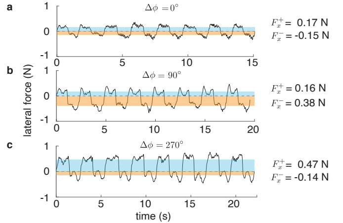
Fig. 9. Symmetric resistance was observed in (a) under a standing wave condition. In contrast, in (b) and (c), higher resistance is observed when the finger slides against the particle motion, compared to when the finger slides in the direction of particle motions. The shaded areas represent the average positive (blue) and negative (orange) forces.
