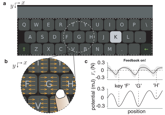
Fig. 10. Demonstration of a haptic keyboard. (a) The user interface displayed on an external screen. Users can interact with the interface by sliding on the flatLoop. (b) Visualization of the desired force fields within the dashed circle. (c) The lateral force measured on a slowly sliding finger across the centerline in the dashed circle area. The graph below shows the calculated potential values derived as the integral of the lateral force. The shaded area represents the standard deviation.
