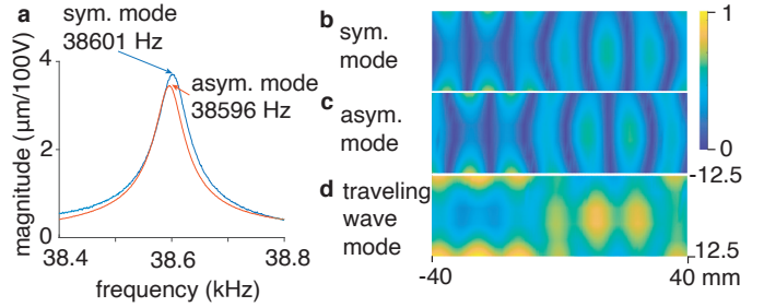
Fig. 6. (a) Experimental frequency response of the two frequency-degenerate modes. (b) Normalized colormaps of the mode shapes of symmetric mode, asymmetric mode, and the resulting traveling wave mode.
