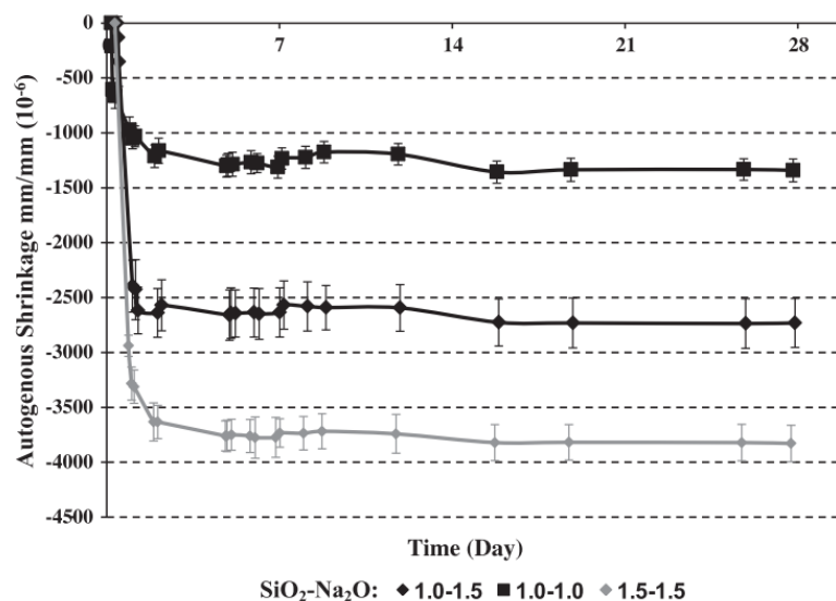
Figure 2.6 Autogenous shrinkage of AAF pastes with different \text{SiO}_2 and \text{Na}_2\text{O} contents, cured at 40 °C [24].
