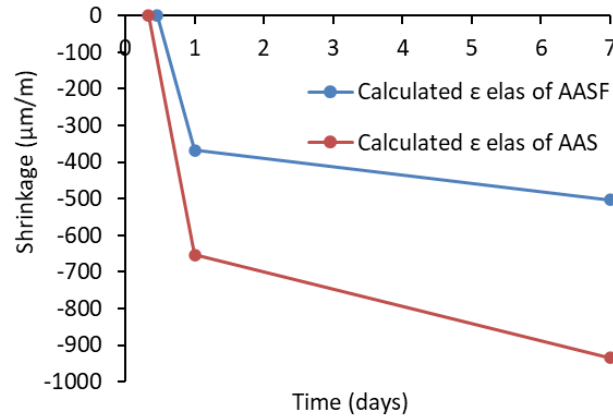
Figure 3.15 Calculated \varepsilon_{elas} of AAS and AASF paste. The time-zero of the curves is the start of the acceleration period of the paste (8 hours and 12 hours for AAS and AASF, respectively).
