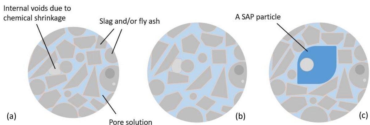
Figure 4.16 Schematic representation of the pore structure of the control paste (a), paste with extra liquid but without internal curing by SAPs (b) and paste with extra liquid with internal curing by SAPs (c).
