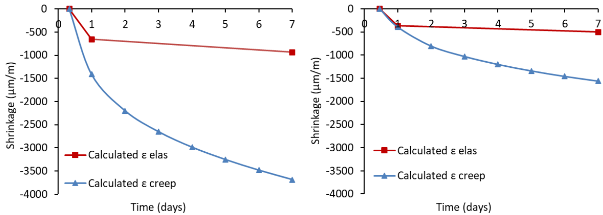
Figure 3.17 Calculated \epsilon_{creep} of AAS (a) and AASF (b) paste, in comparison with \epsilon_{elas} . The time-zero of the curves is 8 hours and 11 hours for AAS and AASF, respectively.
