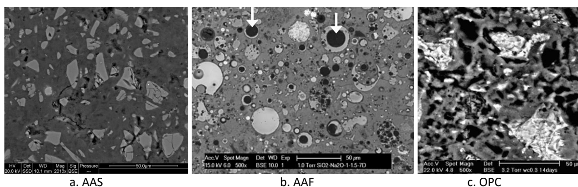
Figure 2.2 (a) BSE images of AAS ( \text{SiO}_2/\text{Na}_2\text{O} = 1.2 , cured at 20 °C for 7 days) [47], (b) AAF ( \text{SiO}_2/\text{Na}_2\text{O} = 0.67 , cured at 40 °C for 7 days) [9], and (c) OPC (water/cement = 0.3, cured at 20 °C for 14 days) [48]. The arrows in (b) indicate the cavities in fly ash.
