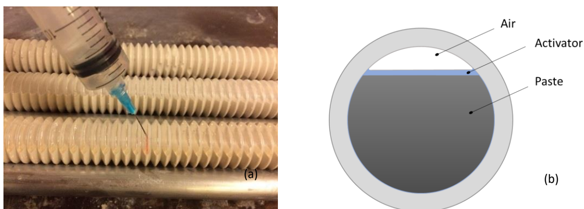
Figure 3.2 Using a syringe to add alkali solution into the corrugated tubes (a) which are 80% filled by the paste (b).
