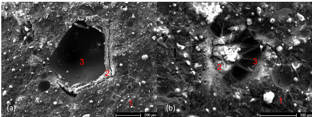
Figure 4.12 SEM images of the SAPs-originated voids in paste AASF0.532SAP cured for 7 days. (a) shows a void that is partly filled by dry SAPs with a big emptied void inside and (b) shows a void that is mostly filled with dry SAPs. The red coloured number 1 indicates the paste, 2 indicates the dry SAPs and 3 indicates the SAPs-originated voids.
