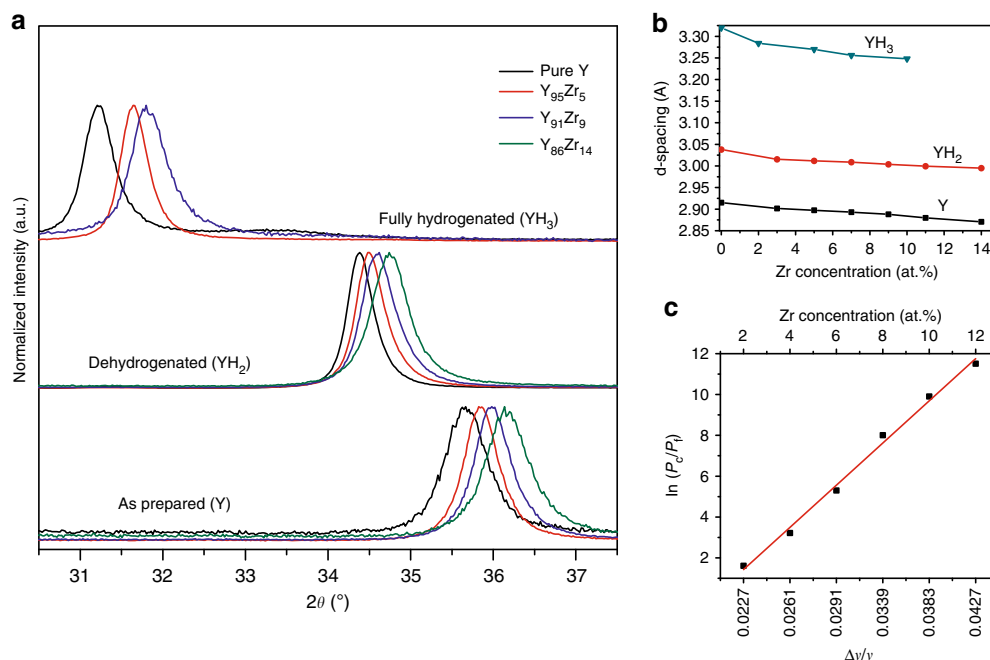
Fig. 2 Lattice behavior of \text{YH}_x as a function of the Zr doping. a XRD pattern of Y-Zr thin films showing the hcp-Y(002) diffraction peak in the as-prepared, fully hydrogenated hcp-YH 3 (002) and dehydrogenated YH 2 (111). The position of the peak clearly depends on the Zr concentration. Note that the Y 86 Zr 14 sample could not be fully hydrogenated to YH 3 even when applying 10 bar H 2 for 24 h. b Change in the corresponding YH x d-spacing as a function of the Zr concentration in the as-prepared, fully hydrogenated (YH 3 ), and dehydrogenated (YH 2 ) state. c Relation between the relative change in molar volume ( \Delta V/V ) of YH 2 and the plateau pressure at the YH 2 ↔ YH 3 phase transition comparing uncompressed ( P_f ) and compressed ( P_c ) YH 2
