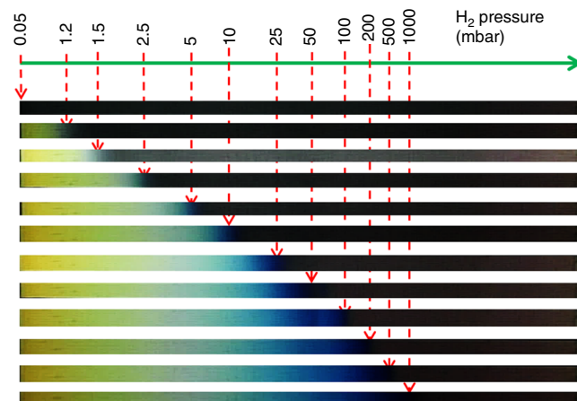
Fig. 5 Visible color changes associated with the formation of YH 3 in a 70 × 5 mm Y 97 Zr 3 –Y 90 Zr 10 gradient thin film. The pictures represent consecutive stages in time of the thin film hydrogenation at different H 2 pressures. The positions of the color front (indicated by the arrows) clearly depend on the hydrogen pressure and Zr concentration. Note that the thickness of the Pd cap layer used for this sample is 50 nm so as to enhance the optical contrast of the film. The sample is viewed from the substrate side
