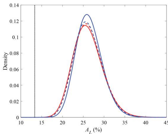
(b) \sigma_e = 0.02
