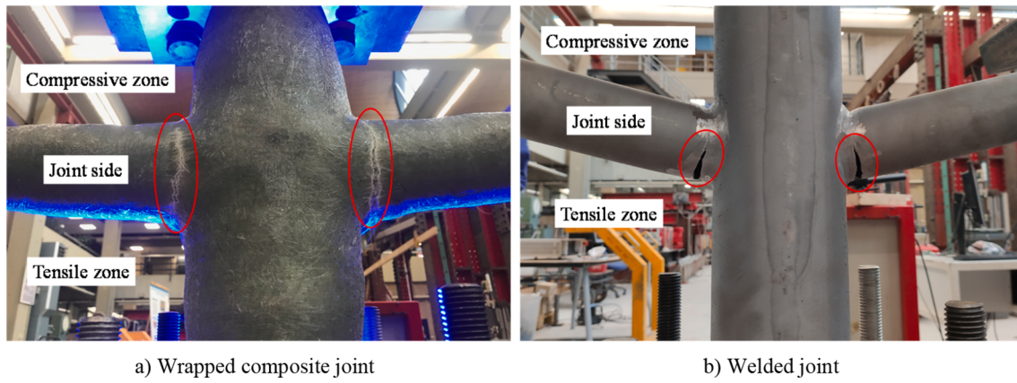
Fig. 22. Failure pattern on 90° small-scale wrapped composite joint specimens vs welded counterparts.
