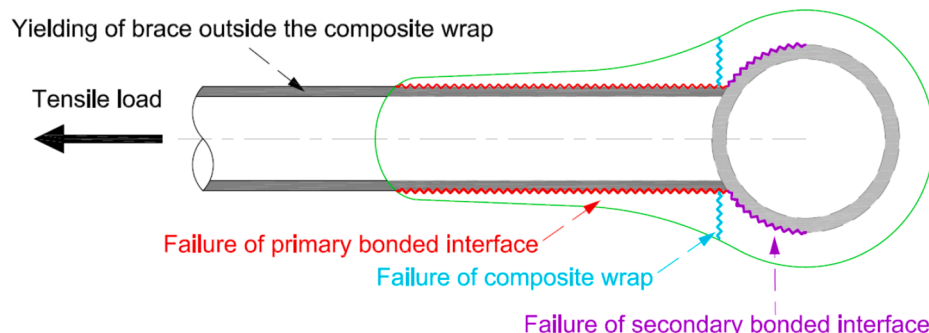
Fig. 7. Load transfer mechanism of a wrapped composite joint loaded in tension.
