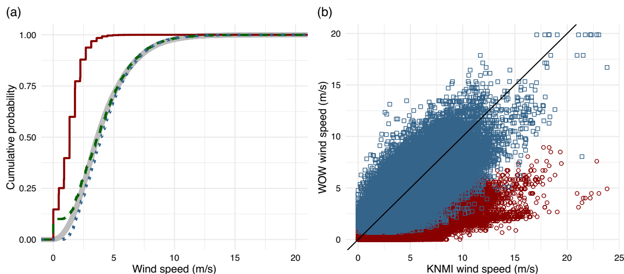
FIGURE 11 QC and BA results of an example WOW station (serial number: 956296001) compared with a KNMI station (Cabauw). (a) Cumulative density distribution of WOW wind speed in raw data (solid line), after the within-station QC and the EQM BA (dashed line), and after the between-station QC and estimating censored low wind speeds (dotted line), with KNMI wind speed (grey thick line) as a reference. (b) Scatter plot of simultaneous observations between the WOW and the KNMI stations, showing both the raw WOW data (circles) and final WOW data (squares) [Colour figure can be viewed at wileyonlinelibrary.com ]
