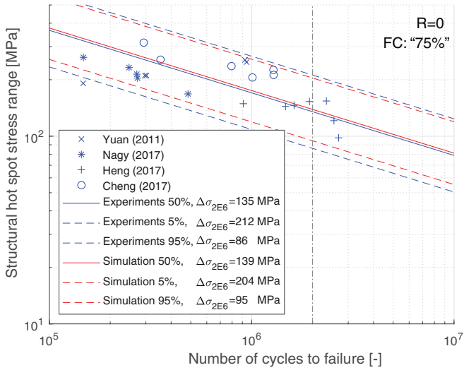
Fig. 26. Comparison of the experimental data and simulated results, R = 0 and FC: "75%".
