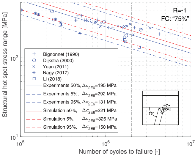
Fig. 31. Comparison of the experimental data and simulated results, Type 2 profile, R = -1 and FC: "75%".
