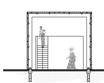
THE GRID VOLUMES (EXAMPLES) 1:200
