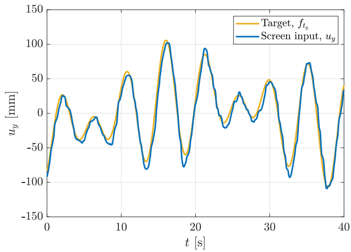
Figure 3. Example target f_{t_y} and touchscreen input u_y time traces for the multisine task.
