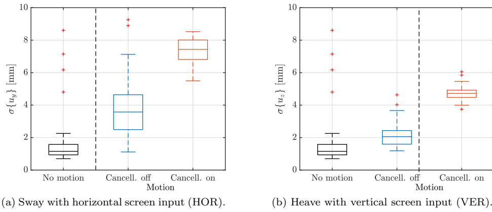
Figure 13. Comparison of step task endpoint variation with and without model-based cancellation.
