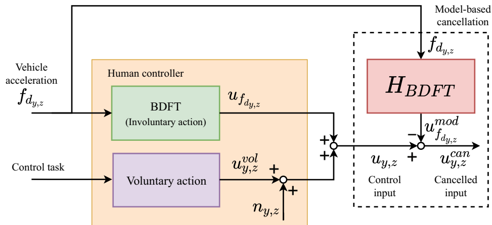
Figure 1. Definition of open-loop BDFT and model-based BDFT cancellation.
