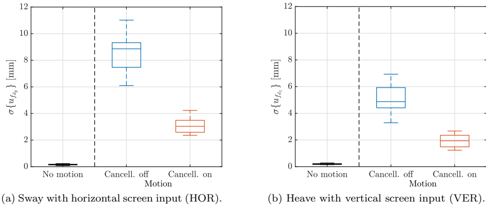
Figure 11. Comparison of the standard deviation of the disturbance component in the input signal \sigma\{u_{f_{d_{y,z}}}\} for the multisine task.
