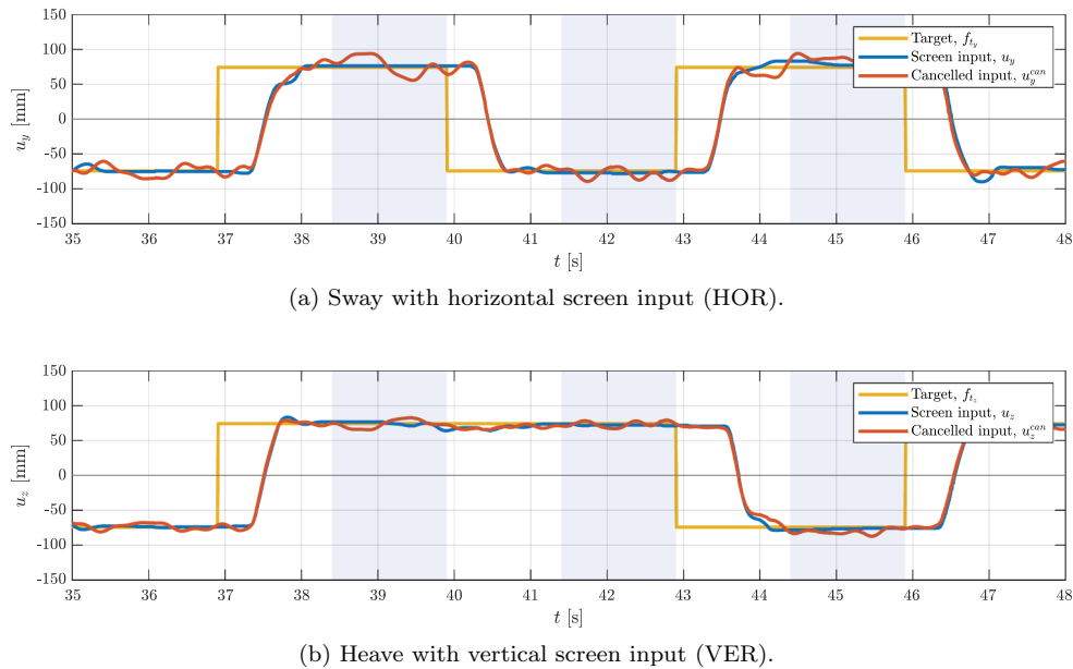
Figure 12. Typical time traces for the step task with BDFT cancellation in both the HOR and VER conditions (Participant 1, Trial 1). The shaded areas indicate the stabilized endpoint data that were used for cancellation assessment.
