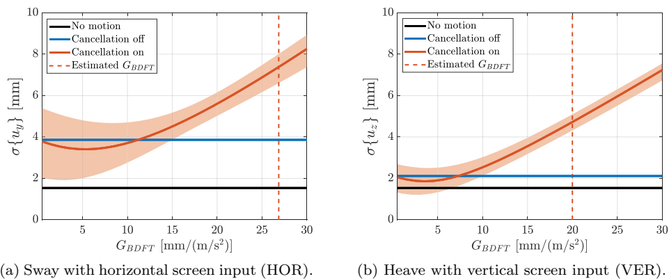
Figure 14. Step task endpoint variation for varying G_{BDFT} .
