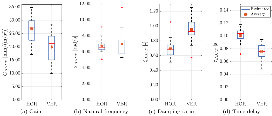
Figure 9. Estimated BDFT model parameters.
