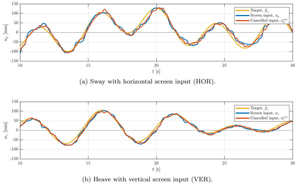
Figure 10. Typical time traces for the multisine task with BDFT cancellation in both the HOR and VER conditions (Participant 1, Trial 1).
