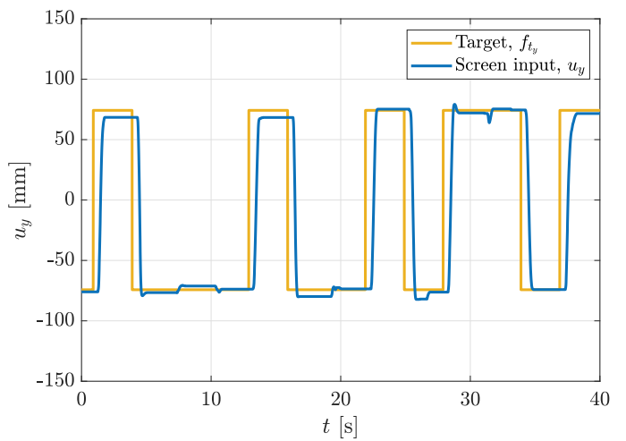
Figure 5. Example target f_{t_y} and touchscreen input u_y time traces for the step task.
