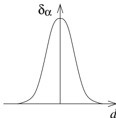
Figure 2.4: Regularized Dirac delta function \delta_\alpha
