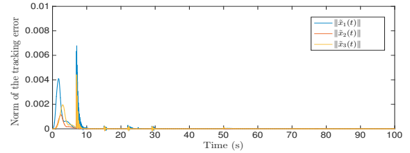
Fig. 4. Norm of the state tracking error of vehicles 1-3: \|\tilde{x}_i(t)\| , i \in S_3
