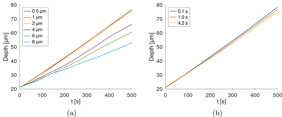
Fig. 2. Mesh and time step size sensitivity analysis of the depth evolution in the pencil test with axial load example: (a) the depths converge to a certain value as the mesh sizes decrease to below 2\mu\text{m} . (b) the depth of specimen in time shows negligible sensitivity to the time step sizes.
