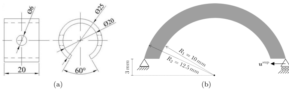
Fig. 9. The C-Ring test set-up: a) geometry and dimensions in mm [16] and b) computational geometry and boundary conditions.
