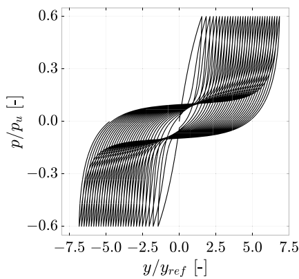
Fig. 13. Cyclic p - y soil reactions (with gapping) under symmetric/two-way loading. Model parameters calibrated based on Eq. (5) for a circular pile (diameter: D = 0.762 m) and a soil location characterized by z = 4 m (soil depth), q_c = 17 MPa (cone resistance), \gamma_{dry} = 16 kN/m 3 (dry unit weight). Additionally: \mu_0 = 20 , \alpha_c = 5 , m_c = 0.6 , and C_d = 0.1 .
