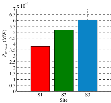
Fig. 6 p_{\text{annual}} for S1~S3 for the optimally-arranged clusters of OPC1
