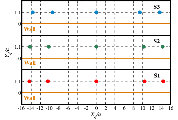
Fig. 7 Optimum layouts of the PAs cluster in front of the wall for S1~S3 and for OPC2
