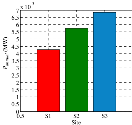
Fig. 10 p_{\text{annual}} for S1-S3 for the optimally-arranged clusters of OPC3
