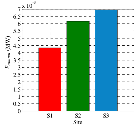
Fig. 8 p_{\text{annual}} for S1~S3 for the optimally-arranged clusters of OPC2
