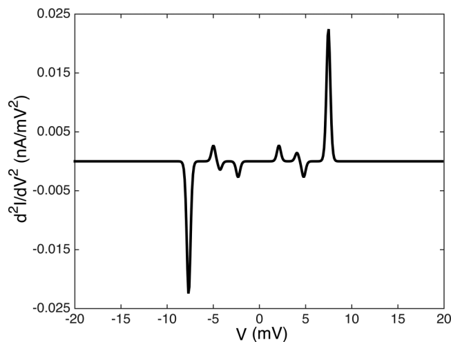
FIG. 6. d^2I/dV^2 spectra corresponding to the differential conductance dI/dV shown in Fig. 4 for E = 0.3 meV.
