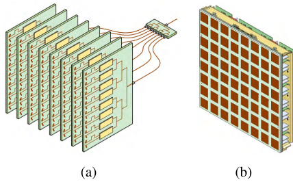
FIGURE 1. Illustration of AESA construction (taken from [42]), (a) traditional approach, (b) planar approach.
