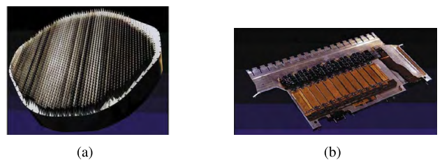
FIGURE 4. An airborne phased array radar antenna (taken from [46]), (a) array aperture, (b) a row of microwave modules on a slat.
