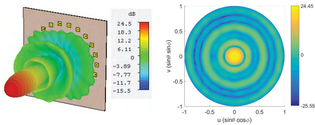
FIGURE 33. Realized gain of the 49-element sparse circular ring array for the broadside beam at 28.5 GHz.
