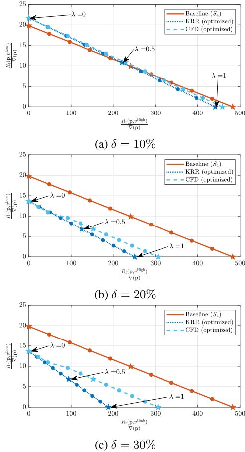
FIGURE 10. Optimization Framework Validation and Physical Plausibility: Pareto frontier ( \frac{R_t(p, v^{High})}{V(p)} on the x-axis and \frac{R_t(p, v^{Low})}{V(p)} on the y-axis) for different values of \lambda and \delta together with the EFD data and the CFD.
