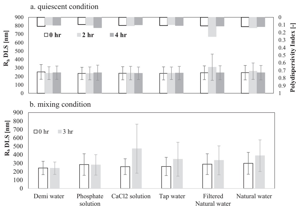
Fig. 2. R_{hDLS} of Si-DNA microparticles in 6 water types as a function of time (a. quiescent condition and b. mixing condition). The error bar represents the standard deviation of the size distribution. Polydispersity index (PDI) is equal to the square of standard deviation of the size distribution divided by the square of the mean.
