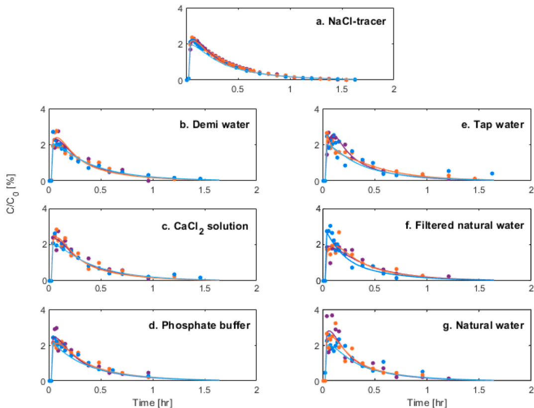
Fig. 3. Observed and simulated BTCs of Si-DNA microparticles in 6 water types plotted in relative concentration C/C_0 [%]. The observed data are shown as solid circles in purple, orange, and blue for the 1st, 2nd, and 3rd replicate experiment, respectively. The corresponding simulated BTC is shown as line in purple, orange, and blue for 1st, 2nd, and 3rd replicate experiment, respectively. The observed and simulated BTCs of NaCl are shown for reference in plot a. (For interpretation of the references to colour in this figure legend, the reader is referred to the web version of this article.)
