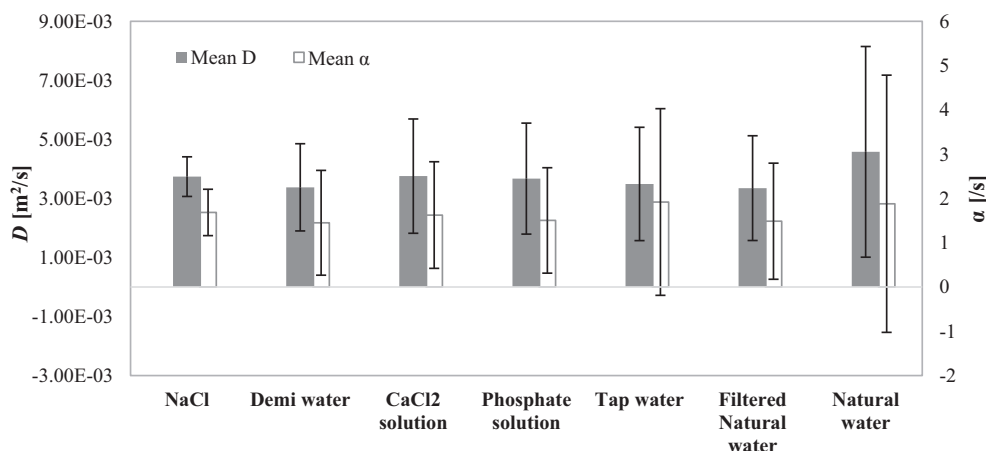
Fig. 4. Mean estimate of D_{Si-DNA} & \alpha_{Si-DNA} in comparison to D_{NaCl} & \alpha_{NaCl} with error bars showing approximate 95% confidence limits.
