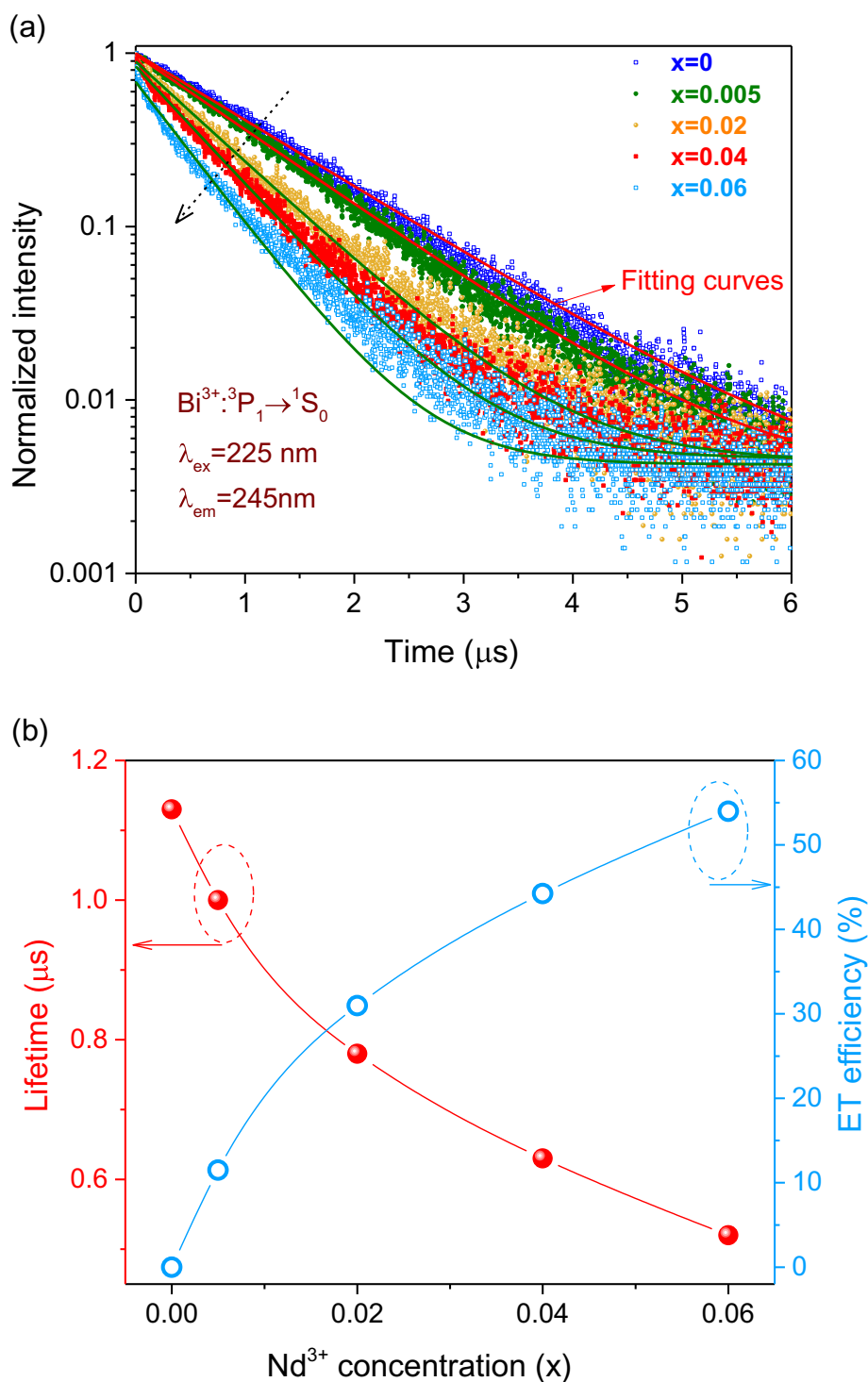
Fig. 4. (a) Fluorescence decay curves and (b) lifetime of \text{Bi}^{3+} A-band emission ( {}^3\text{P}_1 \rightarrow {}^1\text{S}_0 ) at 245 nm upon 225 nm excitation as a function of \text{Nd}^{3+} concentration ( x ) in \text{YPO}_4:0.005\text{Bi}^{3+}, x\text{Nd}^{3+} ( x = 0-0.06 ) recorded at room temperature. The \text{Nd}^{3+} concentration dependence of the energy transfer efficiency of \text{Bi}^{3+} \rightarrow \text{Nd}^{3+} in \text{YPO}_4:0.005\text{Bi}^{3+}, x\text{Nd}^{3+} is shown.
