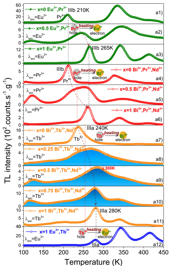
Fig. 11. Low-temperature TL glow curves for \text{Bi}^{3+} and/or \text{Ln}^{3+} doped \text{La}_{1-x}\text{Gd}_x\text{PO}_4 ( x = 0 – 1 ) recorded at a heating of 1 \text{ K/s} after 600 \text{ s} \beta irradiation. A 600 \text{ nm} bandpass filter 600FS40-50 was used to select \text{Eu}^{3+} emission in a1)–a3) and a12), and to monitor \text{Pr}^{3+} red emission in a4)–a6). A 550 \text{ nm} bandpass filter 550FS40-50 was used to monitor \text{Tb}^{3+} green emission in a7)–a11). (For interpretation of the references to colour in this figure legend, the reader is referred to the web version of this article.)
