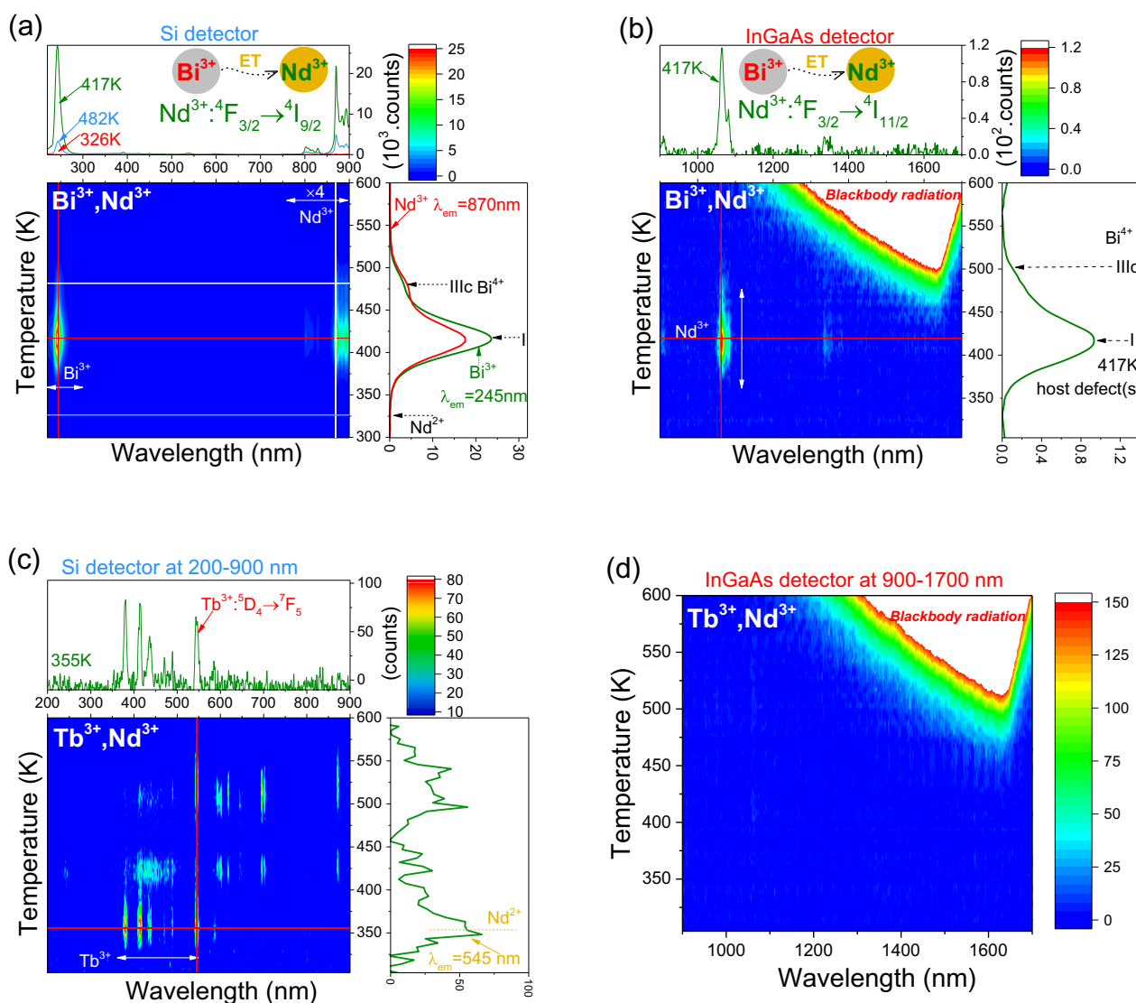
Fig. 6. Thermoluminescence emission (TLEM) plots for (a),(b) \text{YPO}_4:0.005\text{Bi}^{3+}, 0.005\text{Nd}^{3+} and (c),(d) \text{YPO}_4:0.005\text{Tb}^{3+}, 0.005\text{Nd}^{3+} recorded at a heating rate of 1 K/s after \gamma -ray irradiation from a ^{60}\text{Co} source. The emission signal from each sample has been measured using a Si detector QE65000 at 200–900 nm and an InGaAs detector at 900–1700 nm.
