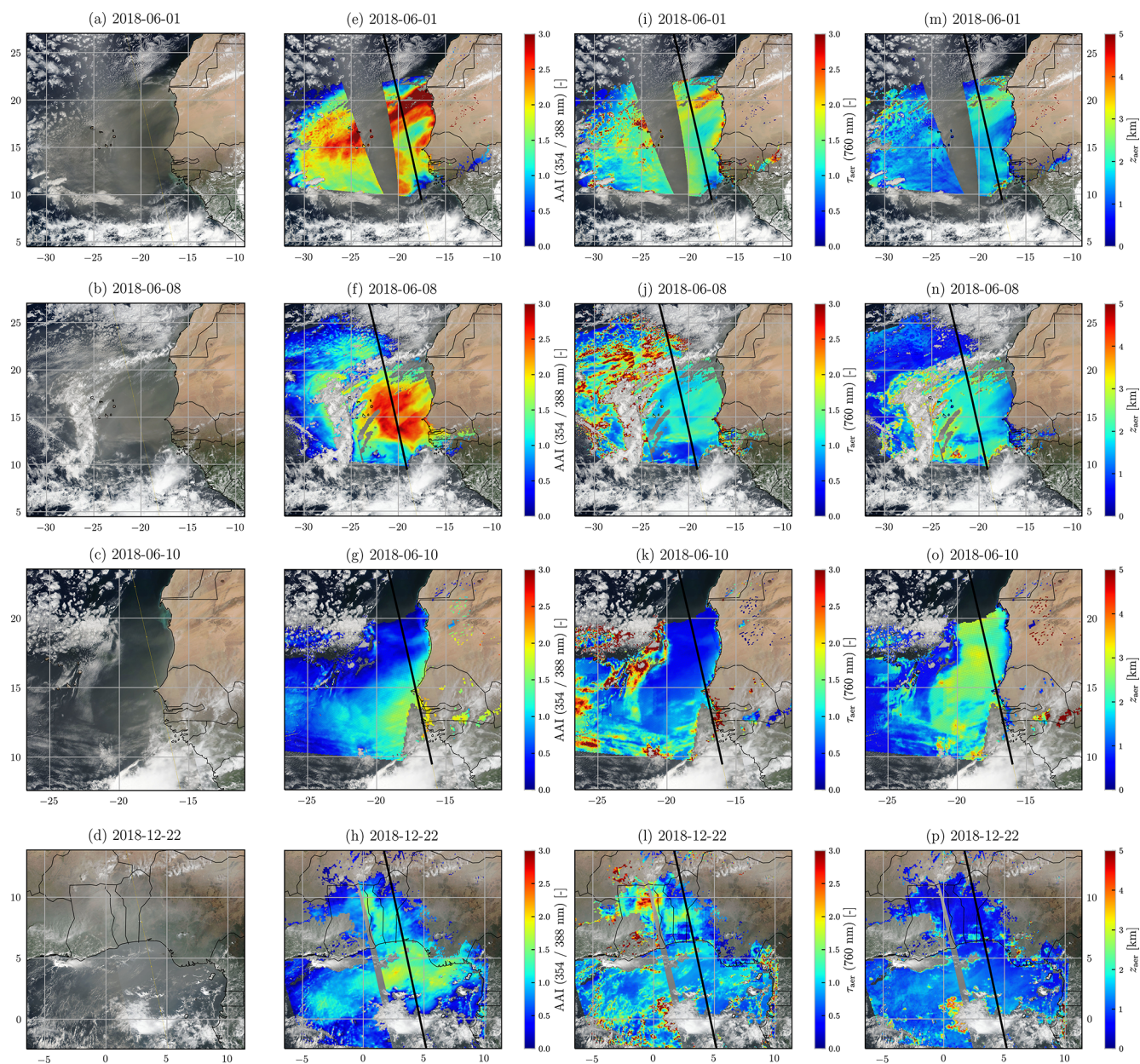
Figure 5. First column: corrected reflectance for the four selected cases as measured by the Suomi NPP/VIIRS imager. The yellow line represents the CALIOP ground track. Second column: the TROPOMI level-2 UV aerosol index product. The black line passing through the TROPOMI level-2 retrievals on this plot represents the ground track of the CALIPSO mission. Third column: retrieved AOT from TROPOMI. Fourth column: operational TROPOMI ALH.
