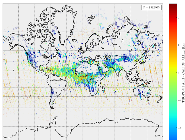
Figure 3. A map of cloud-filtered and sun-glint-filtered differences between co-located TROPOMI ALH and CALIOP ALH ext considered for Fig. 2b.
