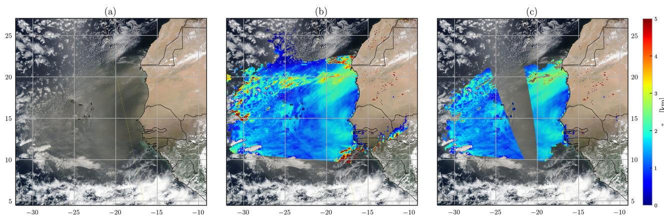
Figure 1. (a) A VIIRS corrected reflectance image over the West African coast on 8 June 2018. (b) All successful TROPOMI retrievals are within a certain bounding box. (c) Same as (b) but with all pixels that possibly fall within the sun-glint region or are cloud contaminated removed (using the cloud_warning flag and sun_glint_warning flag from Table 1).
