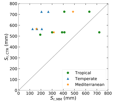
Figure 5. Catchment S_{\text{r}} as estimated from the memory method ( S_{\text{r,MM}} ) compared to the HTESSSEL CTR parameterization ( S_{\text{r,CTR}} ) in the catchment corresponding grid cells.
