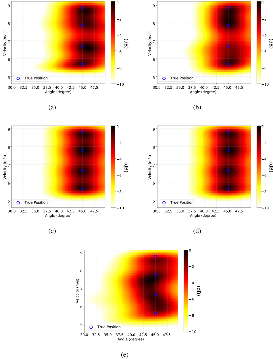
Fig. 3. Angle-Velocity maps of B = 1 GHz and \text{SNR} = 3 dB for (a) 2D MUSIC without phase compensation, (b) 2D MUSIC after Keystone transform, (c) 2D MUSIC with phase compensation and accelerated by Lanczos algorithm, (d) 2D MUSIC with phase compensation and accelerated by Rayleigh-Ritz step and (e) 2D MUSIC with phase compensation and accelerated by inverse algorithm.
