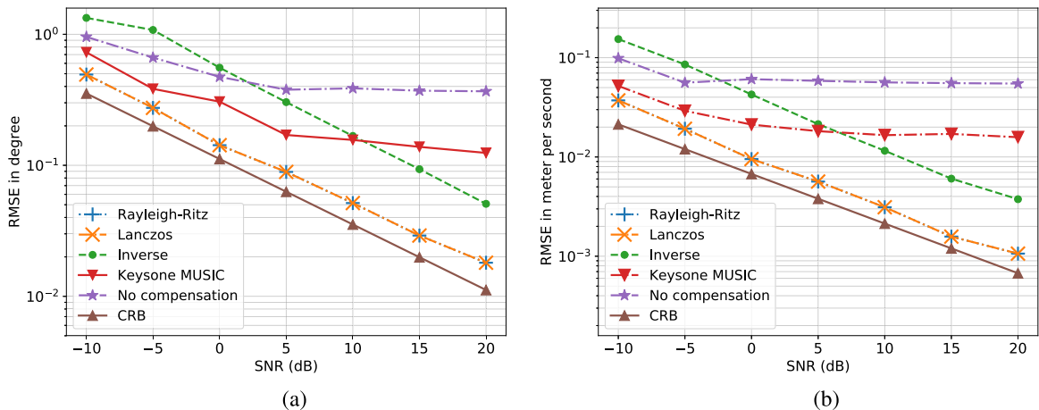
Fig. 2. Comparison of RMSEs with CRLB as a function of SNR at B = 1 GHz for one target at angle 40^\circ and velocity 8 m/s. (a) angle estimation and (b) velocity estimation.
