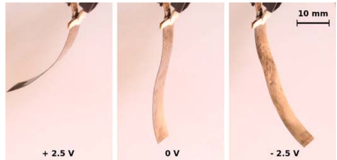
Fig. 1. IPMC actuation: the material at rest (center), and with 2.5 V applied at opposite polarities (left and right).
