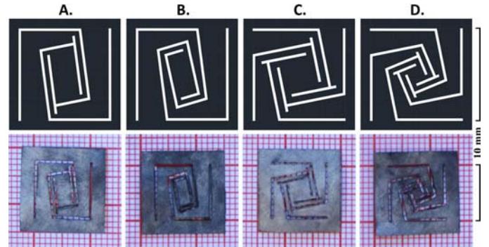
Fig. 5. Designs (top) and realizations (bottom) of the actuation units. We study raising IPMC platform designs with two and four actuator arms with different actuator net lengths.
