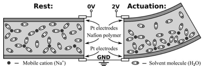
Fig. 2. Simplified explanation of IPMC construction and actuation principles. Ion-conductive polymer (thickness 180 \mu\text{m} in this study) is coated with (10 \mu\text{m} thick) conductive electrodes. Loosely coupled ions migrate in electric field, dragging along solvent. This causes unevenly distributed hydrostatic and Coulomb forces, resulting in bending.
