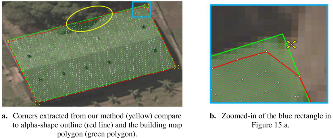
Fig. 15. Corner identification comparison between our proposed method and the reference and the alpha-shape outline in Makassar study area.
