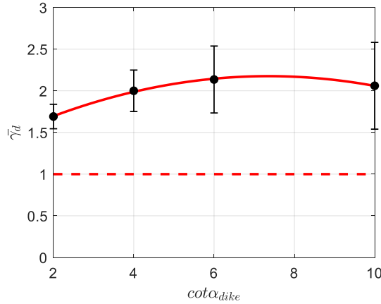
Figure 2.22. Mean response of \tilde{H}_{IG} to variations in \cot \alpha_{dike} , relative to the reference case (no-dike scenario). Red line indicates the model fit (Equation 2.30). Vertical error bars represent the standard deviation of each mean. Dashed red line indicates the mean response obtained for the "no dike" scenario.
