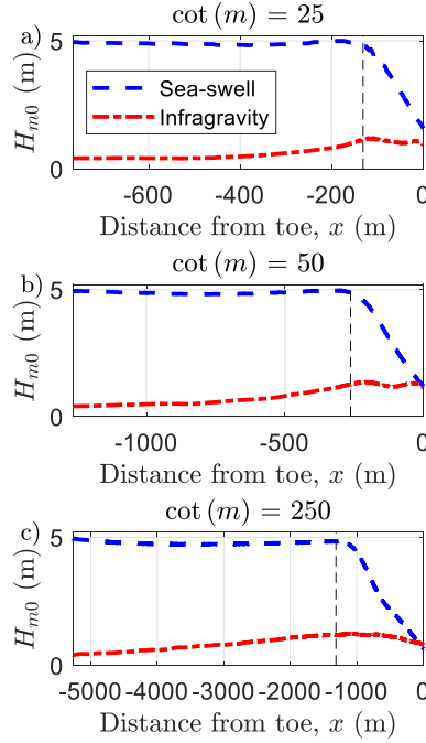
Figure 2.16. Cross-shore profiles of H_{m0,ss} and H_{m0,IG} for (a) \cot(m) = 25 ; (b) \cot(m) = 50 ; and (c) \cot(m) = 250 ( H_{m0,deep} = 5 m, T_p = 11 s, \sigma = 0^\circ , h_{toe} = 1 m, W_{veg} = 0 m and \cot(\alpha) = \infty ). Vertical lines represent the mean break-point location, where h_b = H_{m0}/0.8 .
