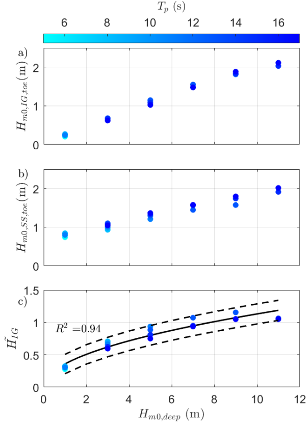
Figure 2.9. Scatterplots of a) H_{m0,IG,t oe} b) H_{m0,SS,t oe} and c) \tilde{H}_{IG} against H_{m0,deep} under reference conditions ( \sigma = 0^\circ , h_{toe} = 1 m, \cot \alpha_{fore} = 50 , W_{veg} = 0 m, n = 0.012 s/m 1/3 and \cot \alpha_{dike} = \infty ), for each of the 24 combinations of H_{m0,deep} and T_p simulated. Solid black line indicates model fit; dashed black lines indicate \pm 95\% confidence intervals.
