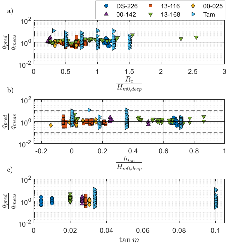
Figure 4.11. Ratio of predicted (Equations 4.29 and 4.35) to measured overtopping discharge versus: a) relative freeboard ( R_c / H_{m0,deep} ), b) relative water depth ( h_{toe} / H_{m0,deep} ) and c) foreshore slope ( \tan m ) for sloping structures (Table 4.2). Solid line indicates perfect agreement. Dashed lines represent predictions that are a factor of 10 higher/lower than measurements. Note that the data for \tan m = 0.029 (1:35 slope) are slightly offset to make all points visible.
