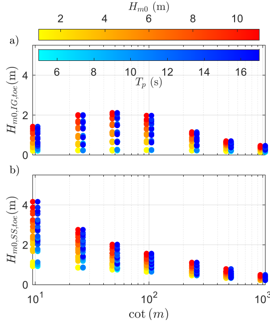
Figure 2.15. Scatterplots of a) H_{m0,IG,toe} and b) H_{m0,SS,toe} against \cot(m) ( \sigma = 0^\circ , h_{toe} = 1 m, W_{veg} = 0 m, n = 0.012 s/m 1/3 and \cot(\alpha) = \infty ). Each data point is represented by two markers with colormaps indicating the magnitude of H_{m0,deep} (hot) and T_p (cold).
