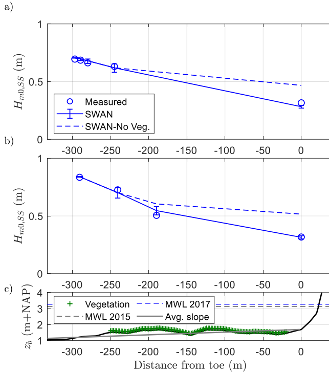
Figure 5.6 Comparison of measured and modelled significant wave heights in the SS bands ( H_{m0,SS} ) at the peaks of the a) January 2015 and b) January 2017 storms at Uithuizerwad (see Figure 5.5 for gauge locations). Error bars represent the uncertainty in the estimates based on the standard deviation of Equation 5.4. Panel 'c' shows the bed level and vegetated cover.
