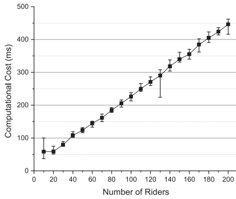
Fig. 7. Computational costs of parallel processing.
