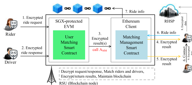
Fig. 3. Collusion-resistant user matching for RHS.
