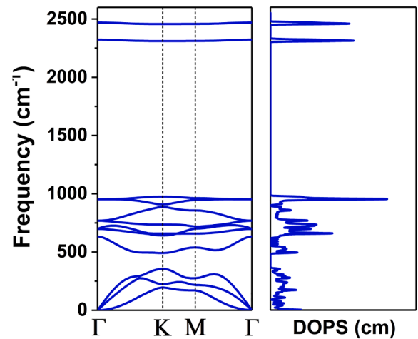
Fig. 1. Phonon frequency dispersions of hydrogenated BP monolayer.
