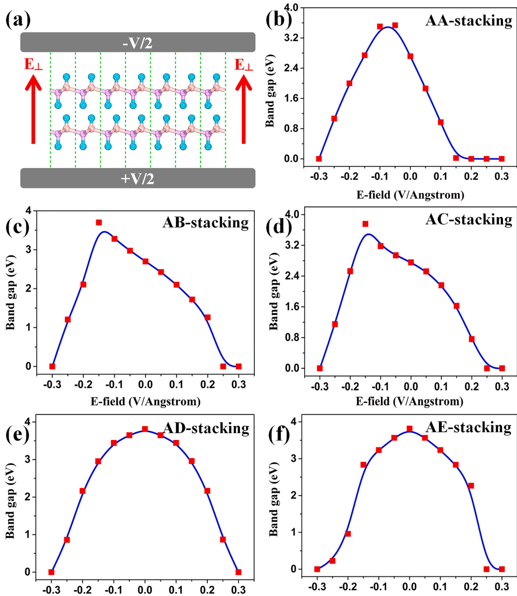
Fig. 5. (a) Schematic illustration of applied E-field in the bilayer hydrogenated BP, where the positive orientation of E-field is donated by red arrows. Vertical E-field dependent bandgap of (b) AA-, (c) AB-, (d) AC-, (e) AD-, and (f) AE-stacked bilayer hydrogenated BP.
