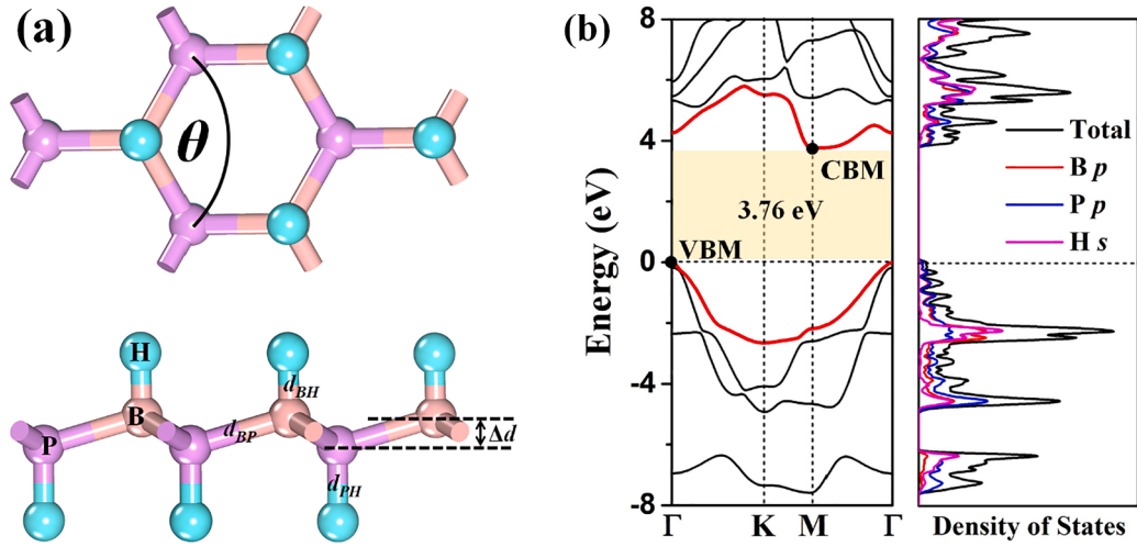
Fig. 2. (a) Top and side view of optimized geometry and (b) the band structures and partial density of states of hydrogenated BP monolayer. The Fermi level is assigned at energy zero.
