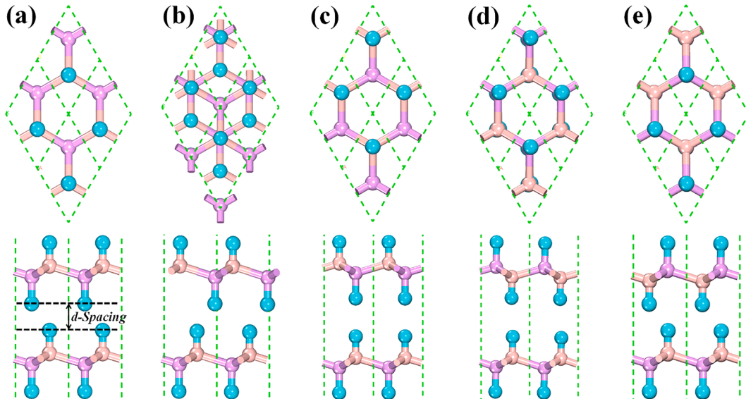
Fig. 3. Five stacking configurations of bilayer hydrogenated BP. Top and side views of the atomic structure of (a) AA-, (b) AB-, (c) AC-, (d) AD-, and (e) AE-stacking with the full relaxation.
