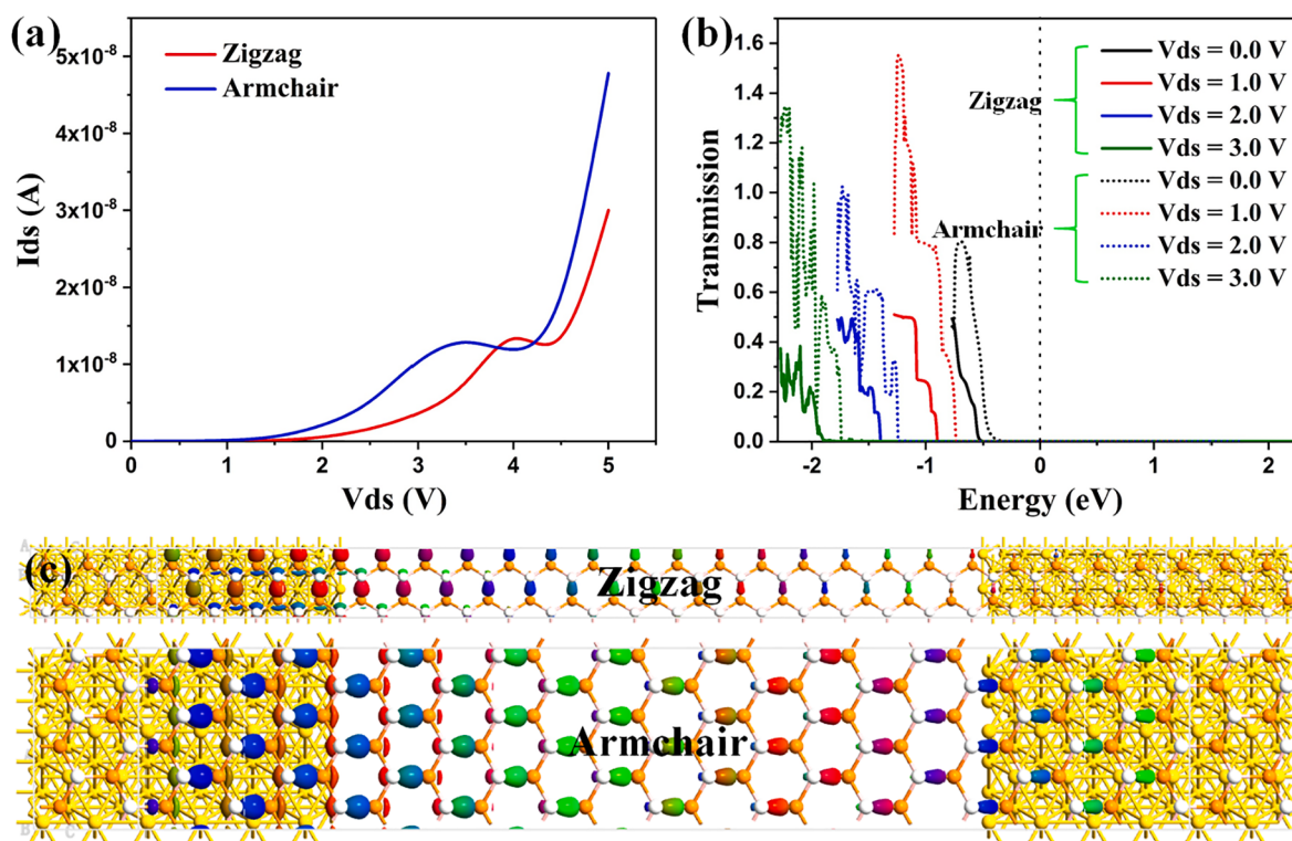
Fig. 8. (a) The I-V characterization and (b) Bias-dependent transmission spectrum of hydrogenated BP monolayer along zigzag and armchair orientations. Isosurface plots of the computed zigzag and armchair directional transmission eigenstates at an energy of -1.0 eV under a bias of 3.0 V are presented in (c). The Fermi level is set to zero.
