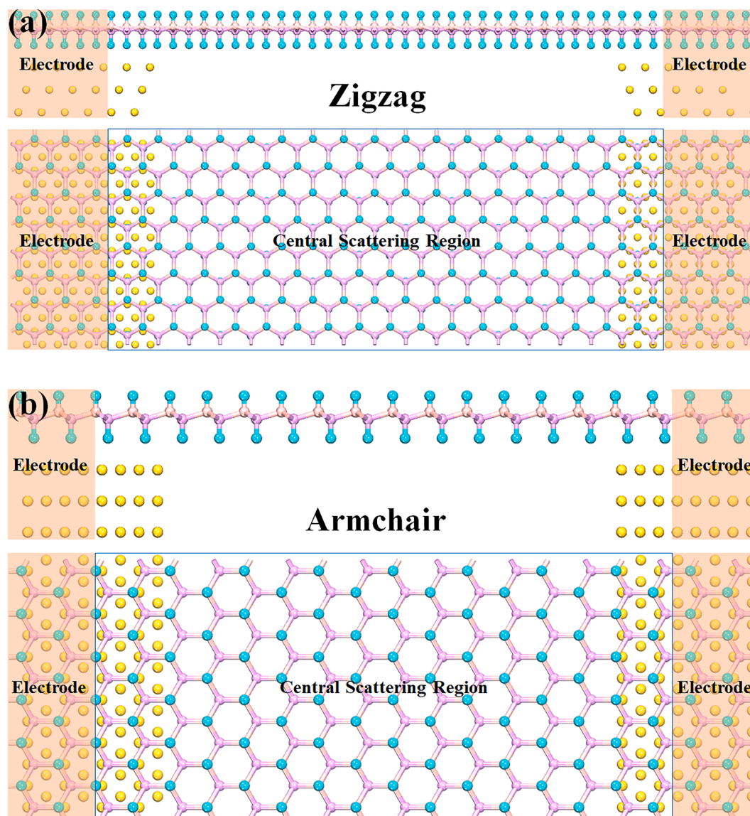
Fig. 7. Schematic representation of the two-probe configurations where metallic atoms (orange shade region) are acted as the semi-infinite left and right electrodes that are in contact with the central scattering region along the zigzag and armchair orientations.
