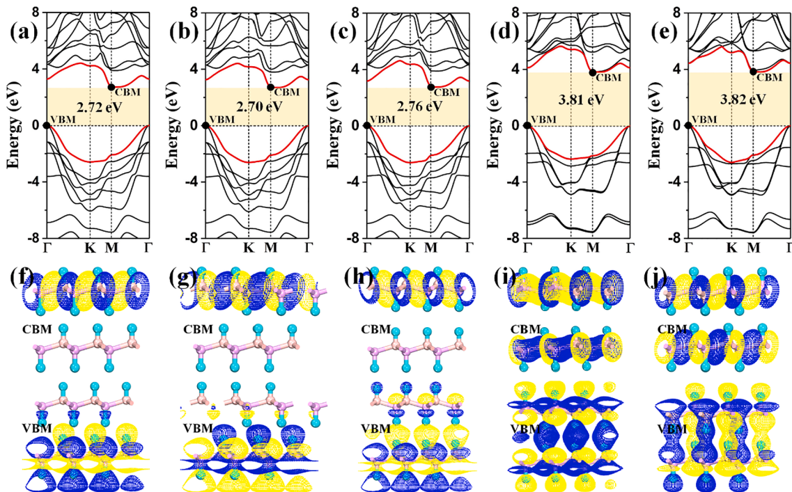
Fig. 4. Calculated band structures of (a) AA-, (b) AB-, (c) AC-, (d) AD-, and (e) AE-stacked configurations and (f, g, h, i, j) the isosurface plot of charge density corresponding to CBM and VBM of AA-, AB-, AC-, AD-, and AE-stacking. The isovalue is taken as 0.03 \text{ e}/\text{\AA}^3 . The Fermi level is set to be 0 eV.
