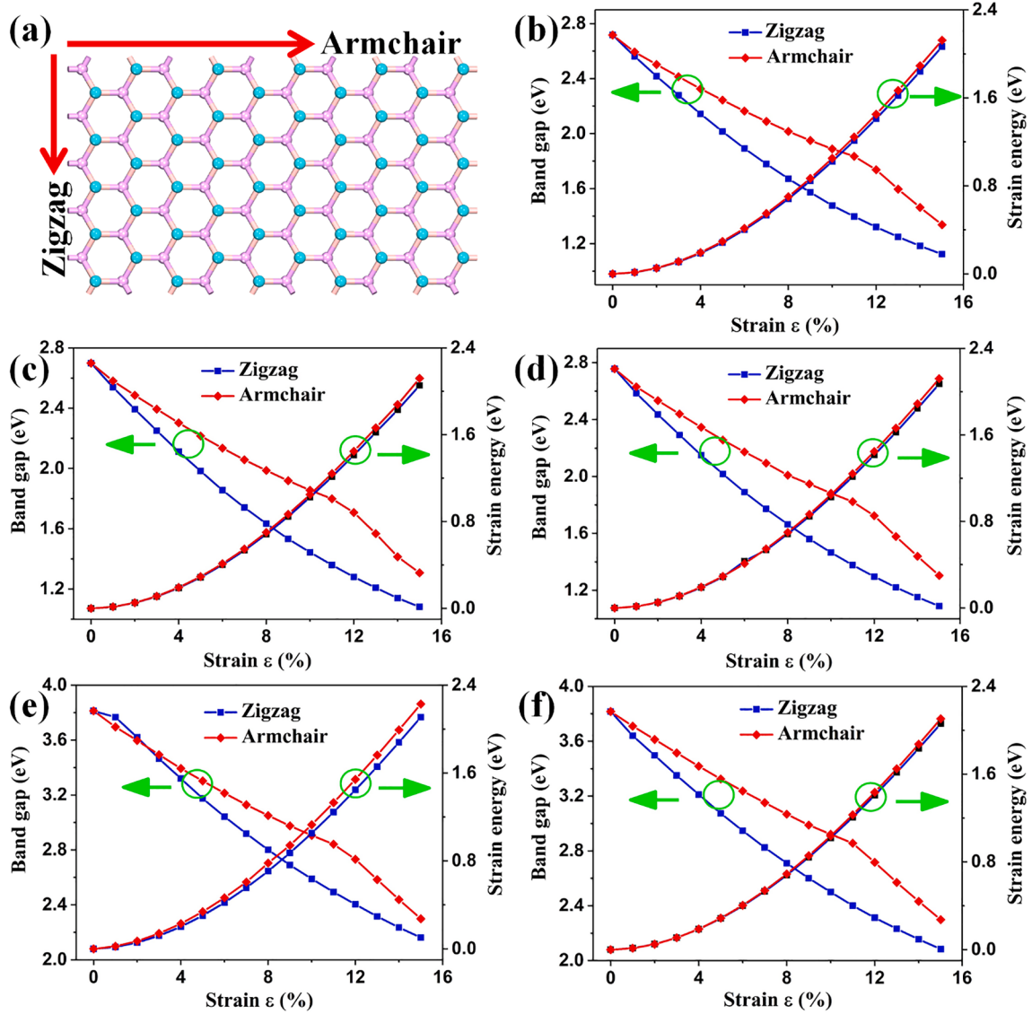
Fig. 6. The electronic properties of five stacked configurations varied with tensile strain. (a) Two directions of tensile strain applied in the different stacking orders. The variation of bandgap and strain energy of (b) AA-, (c) AB-, (d) AC-, (e) AD-, and (f) AE-stacked conformations as a function of tensile strain in the armchair and zigzag directions.
