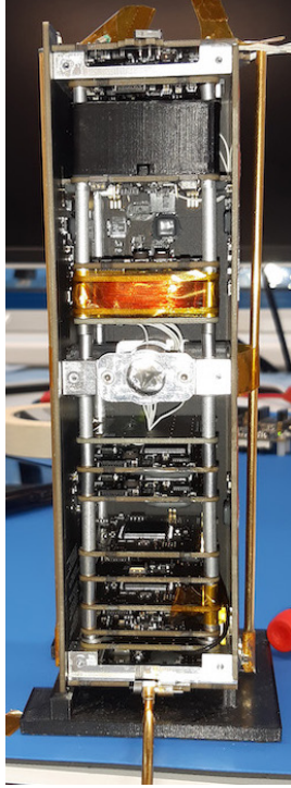
Fig. 5. Delfi-PQ interval view (-X panel removed), subsystem stack (upside down).
