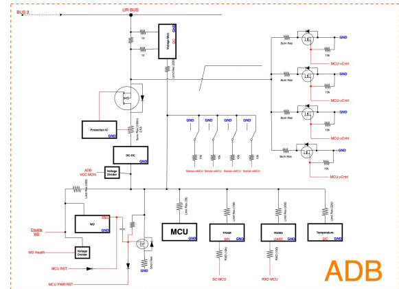
Fig. 11. ADB Block Diagram.
