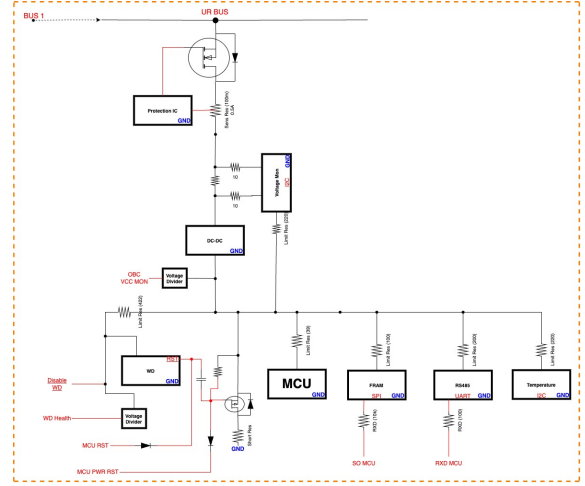
Fig. 6. Delfi-PQ, core electronics block diagram.
