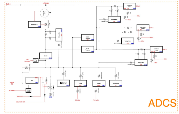
Fig. 10. ADCS Block Diagram.
