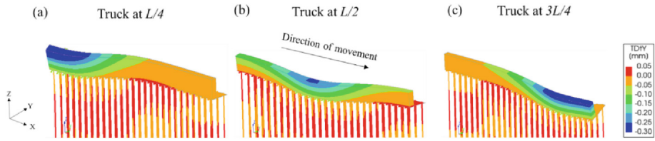
Fig. 6. Out-of-plane displacements of the quay wall during the passage of the fire-truck at different instants: (a) truck at L/4 ; (b) truck at L/2 and (c) truck at 3L/4 . (Deformation scale factor = 2000).
