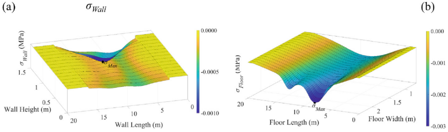
Fig. 4. Normal stress distributions at the instant of occurrence of maximum net compressive force ( \sigma_{Max} ) at: (a) masonry quay wall ( \sigma_{Wall} ) and (b) timber floor for a fire truck ( \sigma_{Floor} ).
