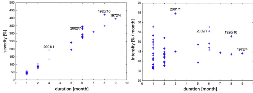
FIGURE 4.12 Duration versus severity ( left ) and duration versus intensity ( right ) of spatiotemporal events in India based on DRASTIC methodology. Some of the most severe events are indicated.
