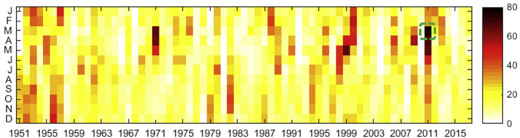
FIGURE 4.7 Percentage of drought area (PDA) for the period 1951–2017 based on SPI6. It is indicated that the highest PDA is in March 2011 (details in Fig. 4.8).
