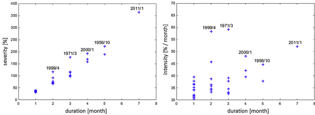
FIGURE 4.6 Duration versus severity ( left ) and duration versus intensity ( right ) of spatiotemporal events in Mexico based on DRASTIC methodology. Some of the most severe events are indicated.
