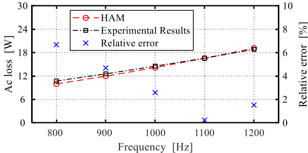
Fig. 9. Comparison of the HAM with the experimental results under ac current input ( I_{\text{rms}} = 20 A).
