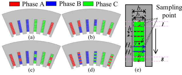
Fig. 1. Illustration of different conductor arrangements in hairpin windings. (a) Conductor arrangement a . (b) Conductor arrangement b . (c) Conductor arrangement c . (d) Conductor arrangement d . (e) Illustration of 1-D ac loss computation model.
