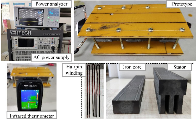
Fig. 8. AC loss measurement experiment.
