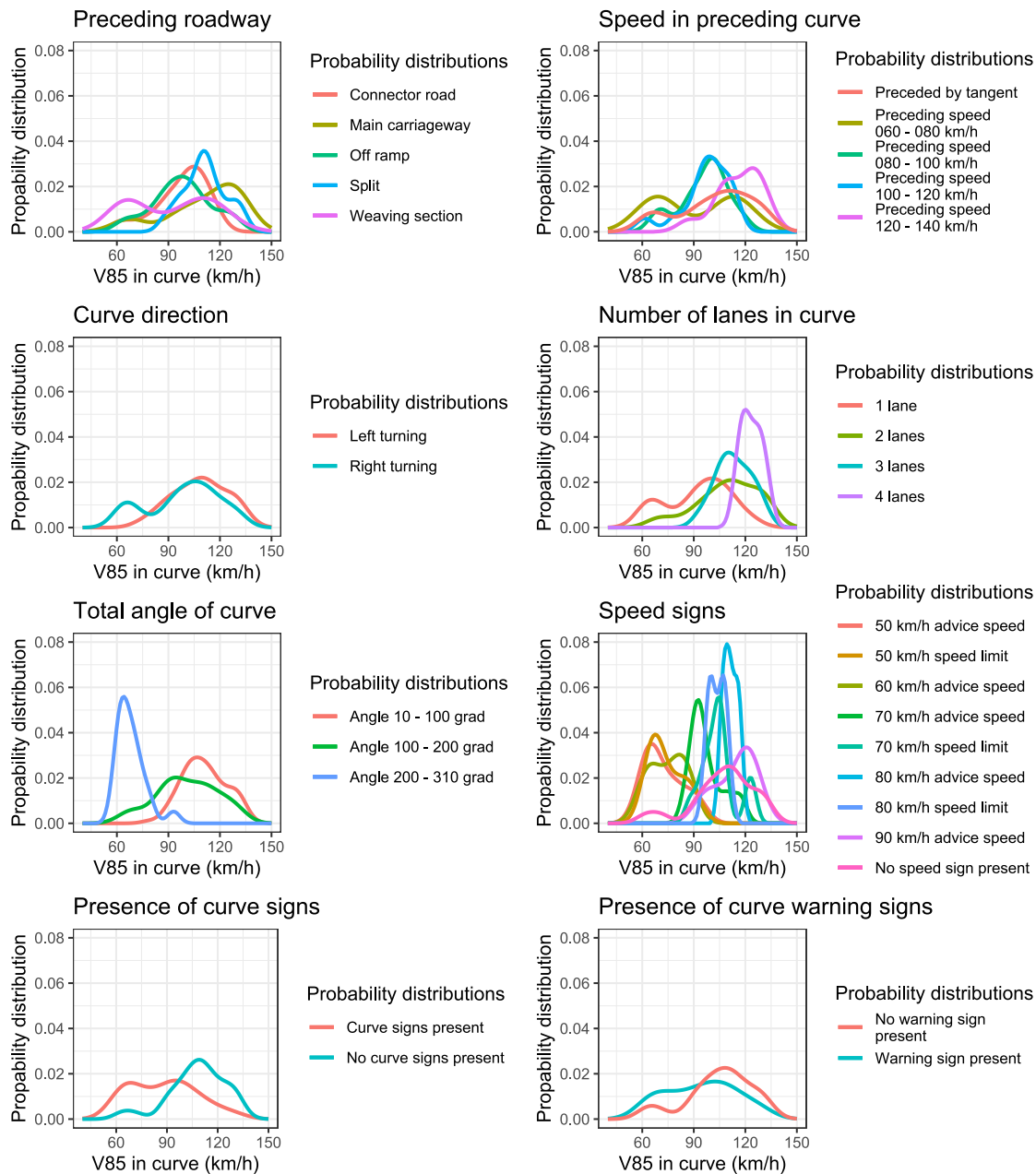
Fig. 5. Probability distributions for the eight different variables (cues) related to the 85th percentile measured median speeds in a curve.
