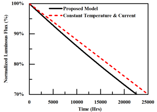
Fig.12 Normalized Luminous Flux in The CCM Mode
