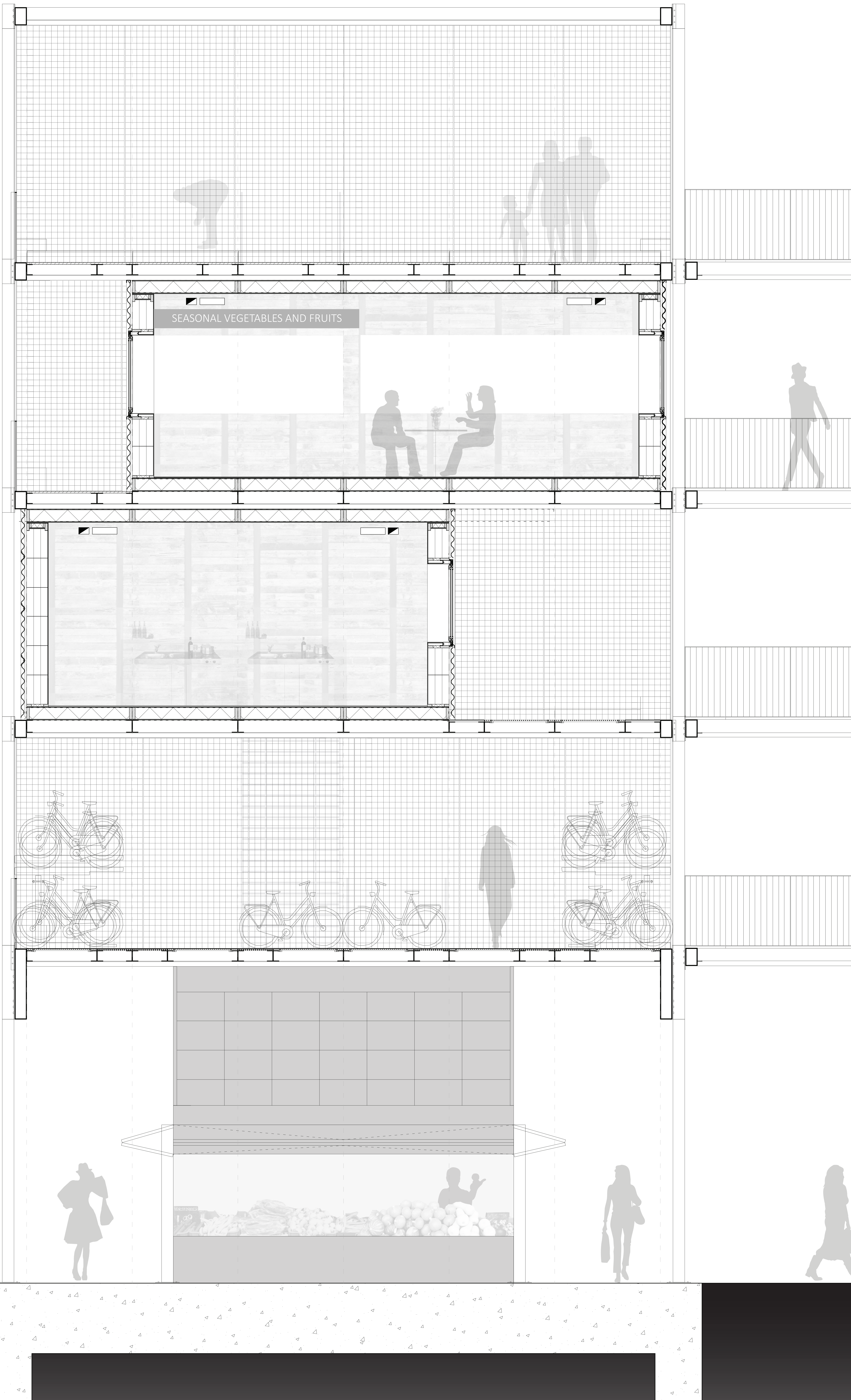
CROSS SECTION 1:20
