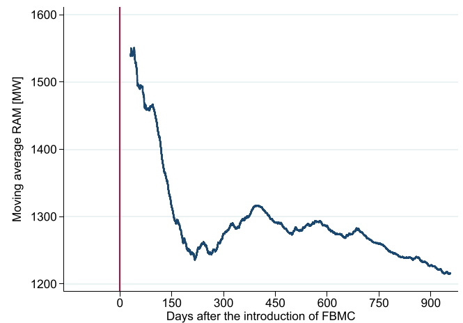
Fig. 6. The average remaining available margin (RAM) in CWE, defined as the sum of RAMs over all reported critical branches divided by the amount of critical branches in that hour, for gradually increasing sample periods after the introduction of FBMC. The moving average first steeply decreases in the four months after the introduction of FBMC and then stay approximately constant.
