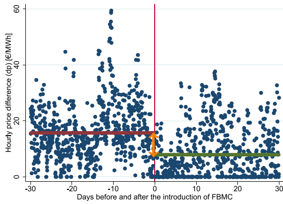
(a) Pre/post. \beta_{FBMC, \Delta P} = -7.8 €/MWh.
